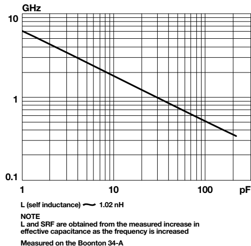
Typical Self Resonant Frequency vs. Capacitance Accu-P® 1210
