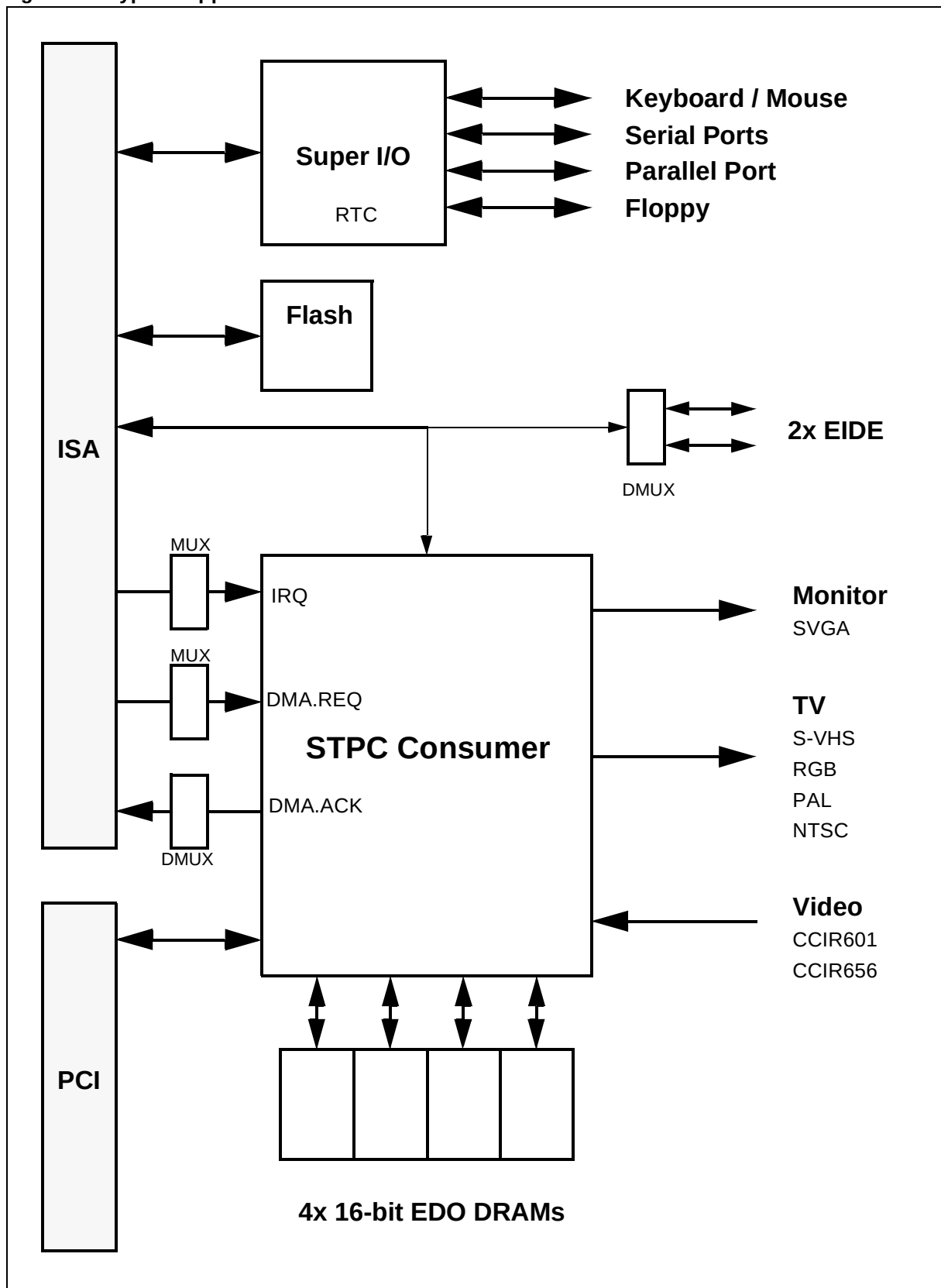
Figure 1-2 Typical Application
