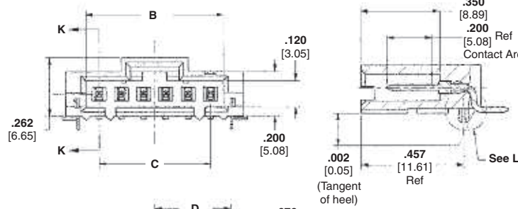
Section K-K
