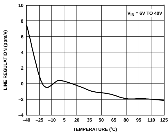
Figure 19. ADR06 Line Regulation vs. Temperature
