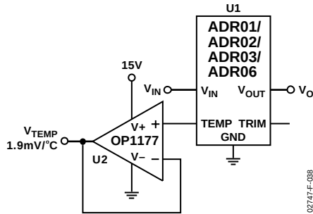
Figure 38. Temperature Monitoring
