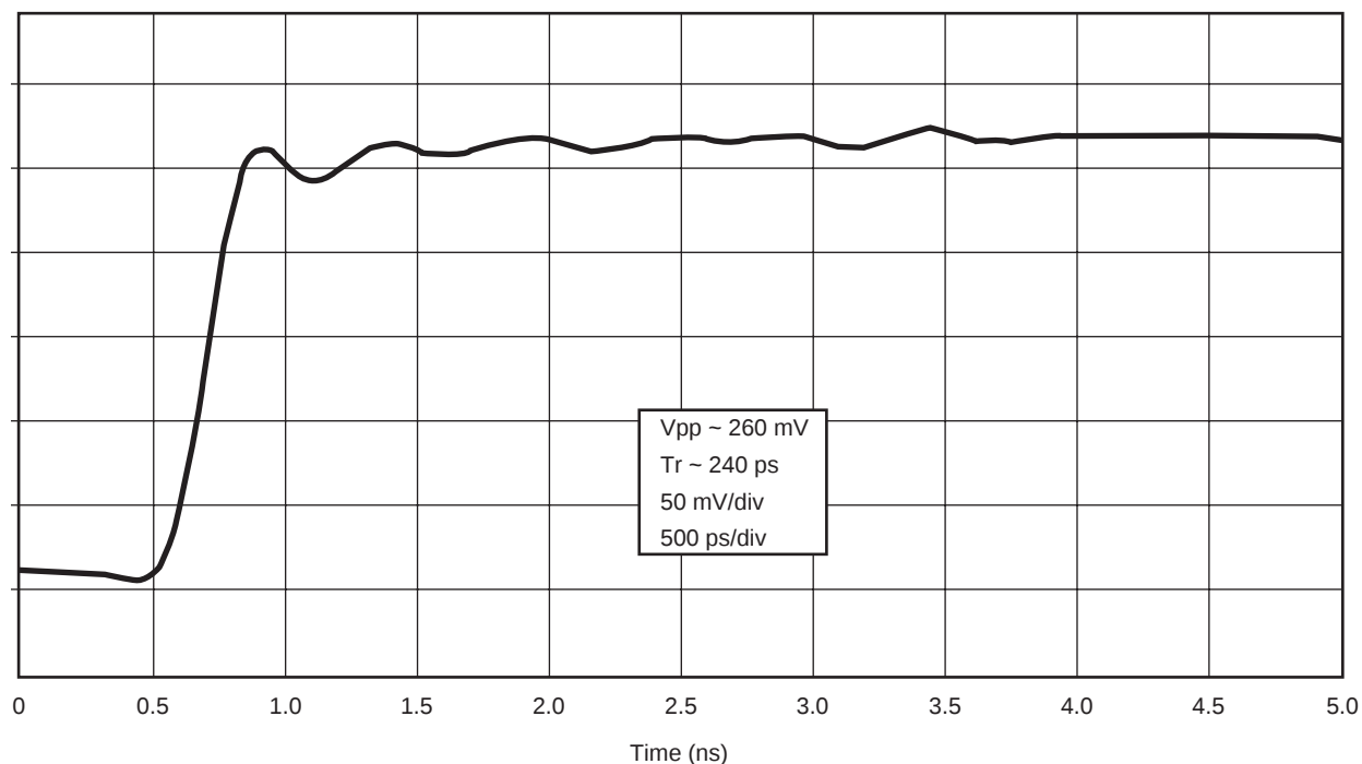
Figure 27. Test Pulse Digitized with 20 GHz DSO
