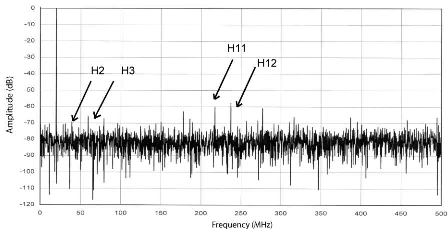
Figure 11. F_S = 1 GSPS; F_{IN} = 20 MHz
