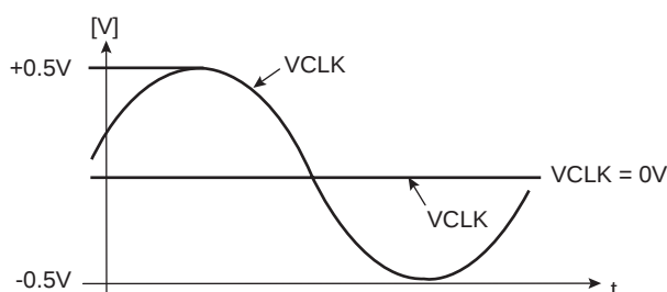
Figure 31. Single-ended Clock Input (Ground common mode):
