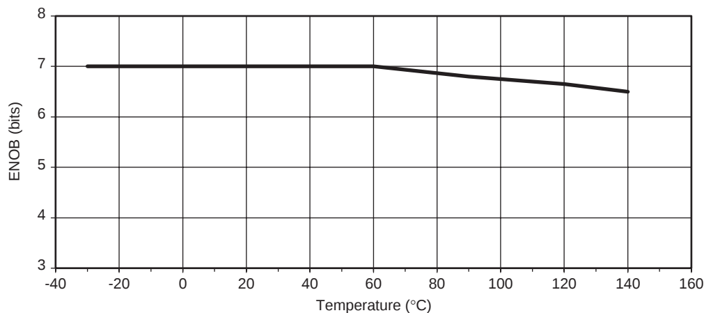
Figure 22. Signal to Noise Ratio Versus Junction Temperature
