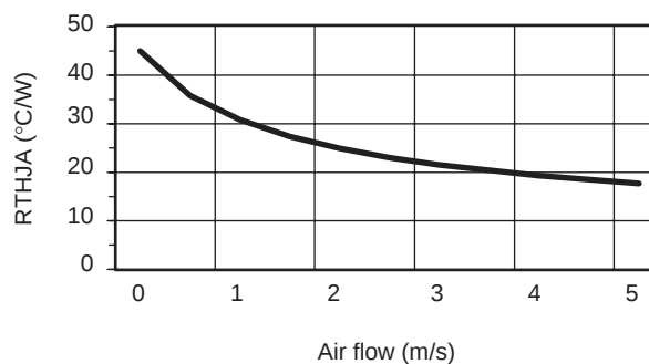
Figure 48. Thermal Resistance from Junction to Ambient: RTHJA
