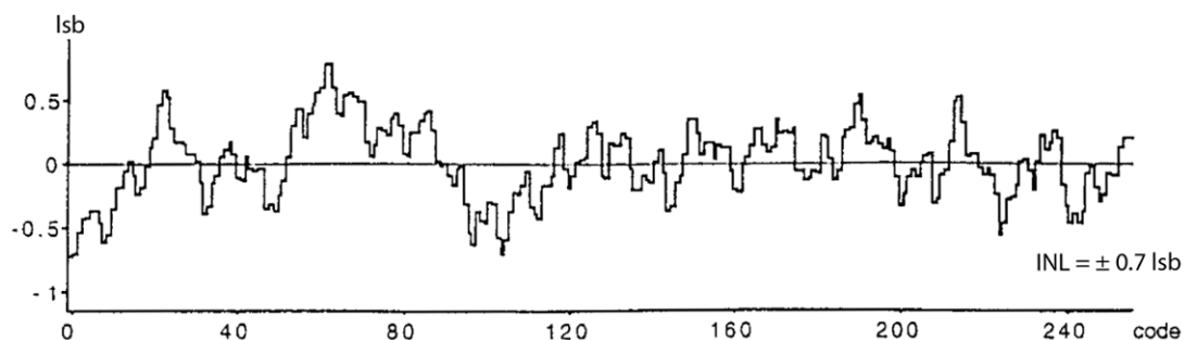
Figure 6. Integral Non Linearity
