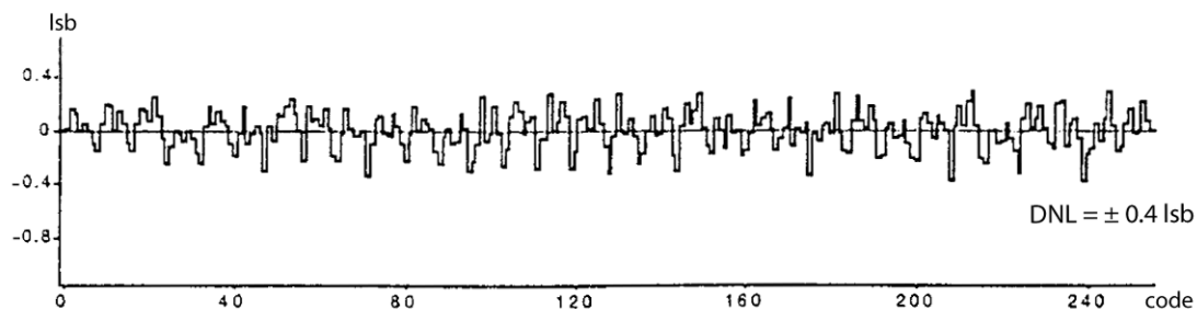
Figure 7. Differential Non Linearity
