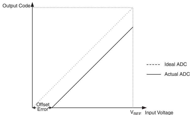
Figure 21-10. Offset Error
