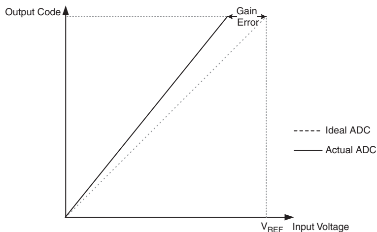
Figure 21-11. Gain Error
