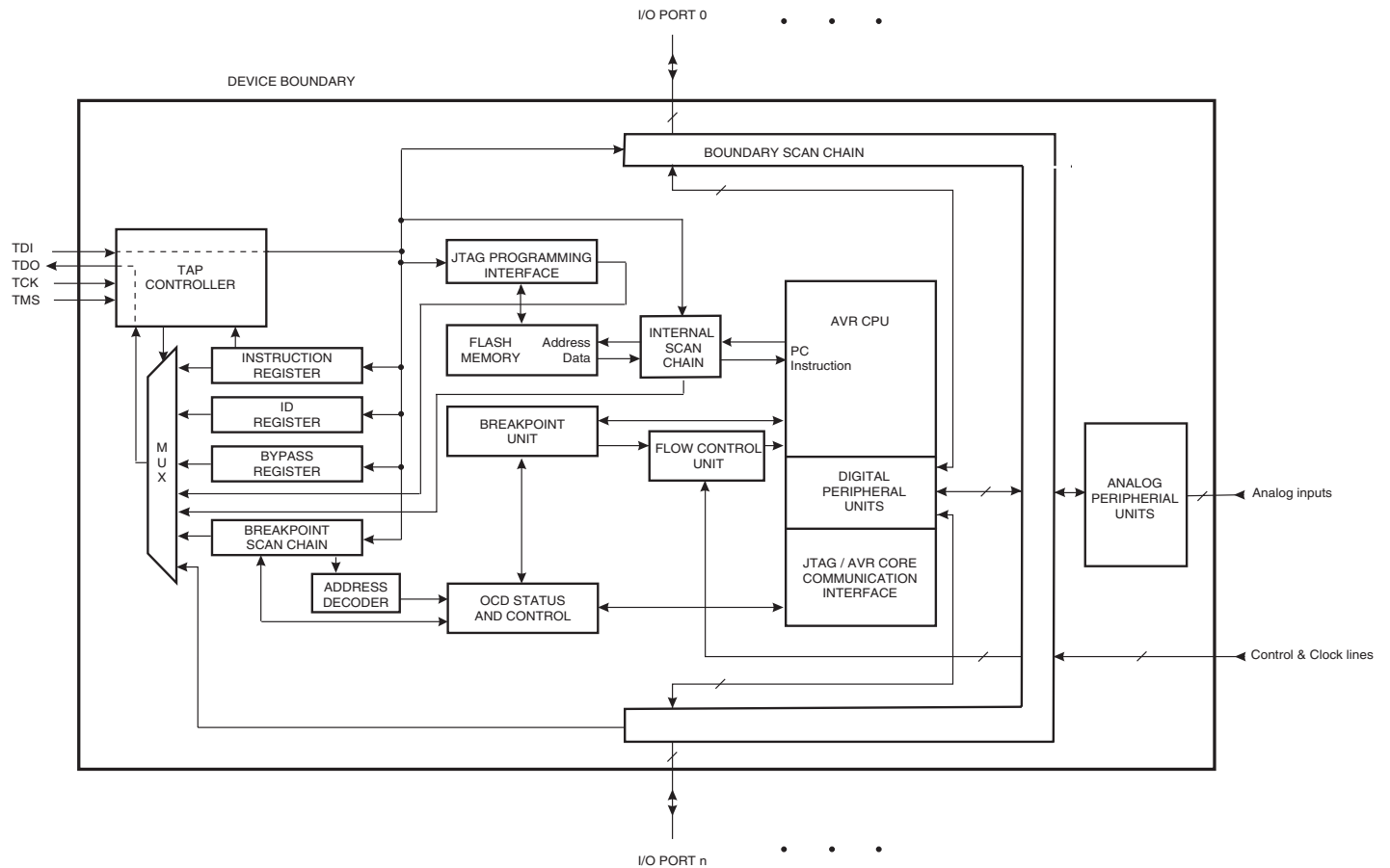
Figure 22-1. Block Diagram
