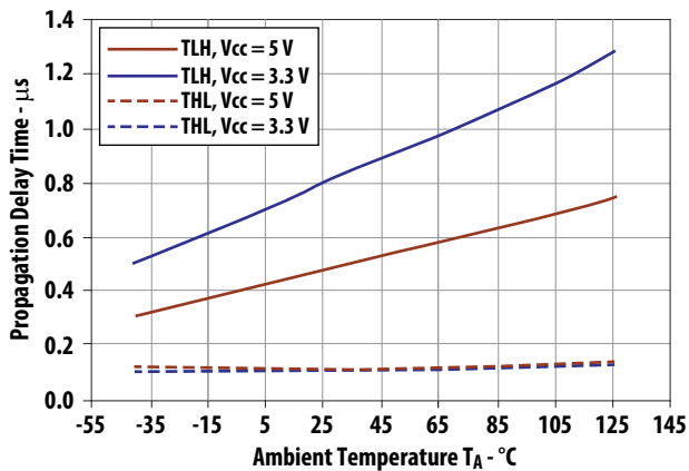
Figure 5: Propagation Delay Time vs. Temperature.
