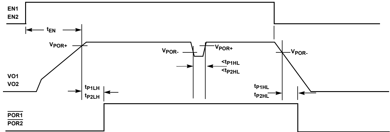
FIGURE 2. TIMING PARAMETER DEFINITION
