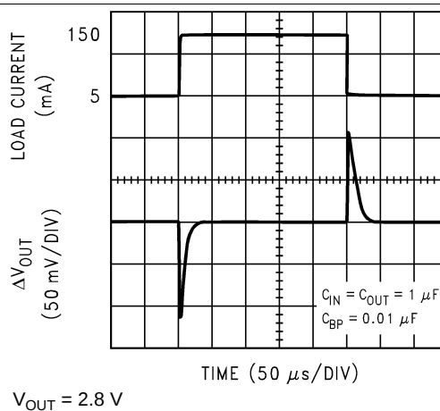
Figure 20. Load Transient Response
