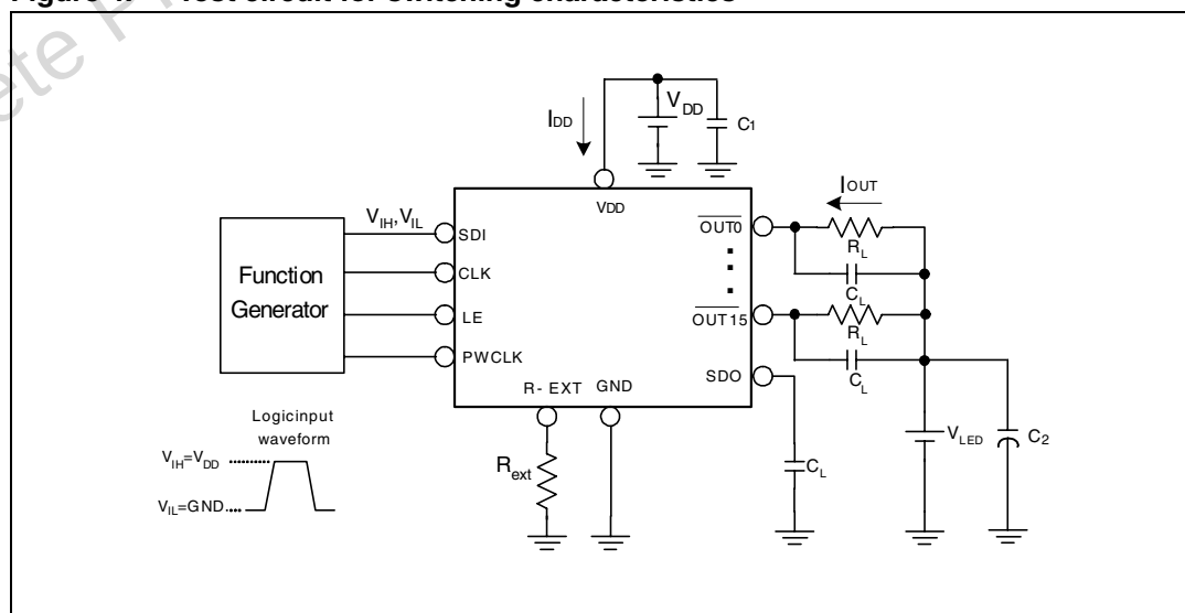
Figure 4. Test circuit for switching characteristics
