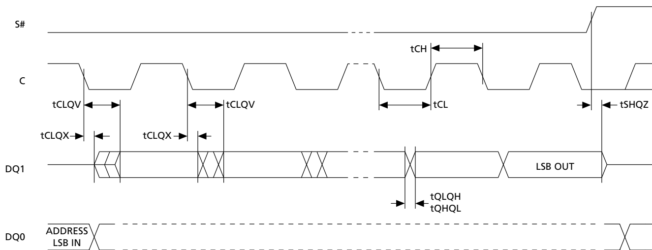
Figure 34: Output Timing
