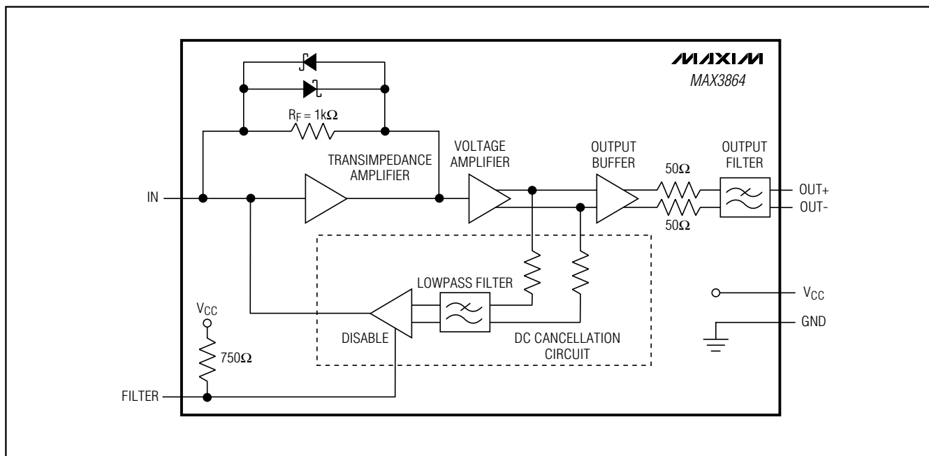
Figure 1. Functional Diagram
