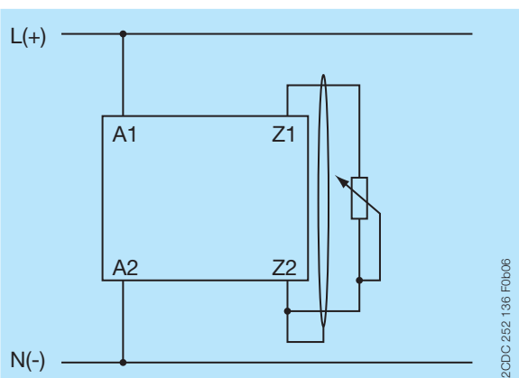
Remote potentiometer
