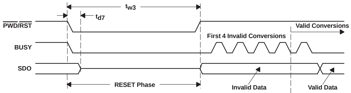
Figure 4. Device Reset
