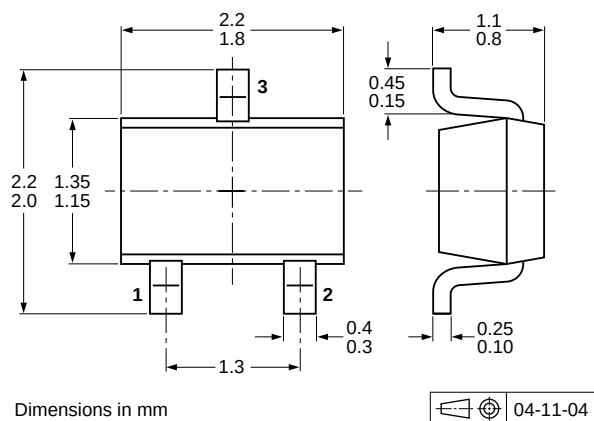
Fig 15. Package outline PDTA143EU (SOT323/SC-70)
