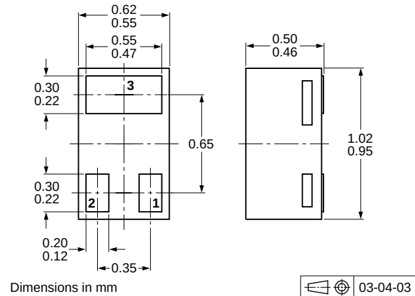
Fig 13. Package outline PDTA143EM (SOT883/SC-101)
