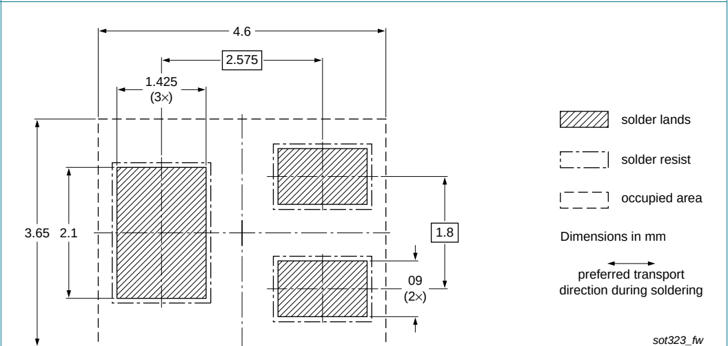
Fig 20. Reflow soldering footprint PDTA143EU (SOT323/SC-70)
