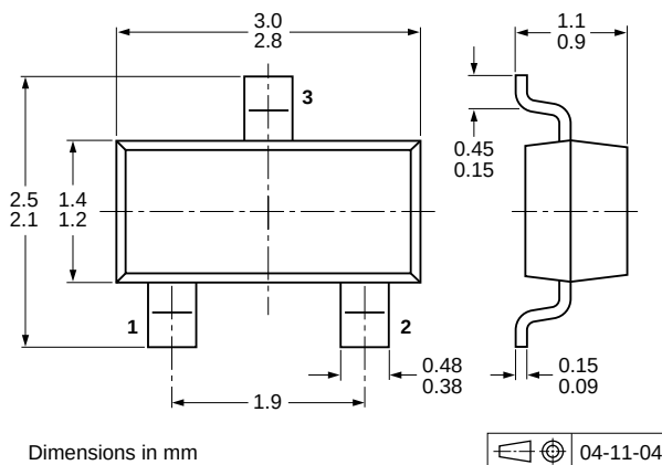
Fig 14. Package outline PDTA143ET (SOT23)
