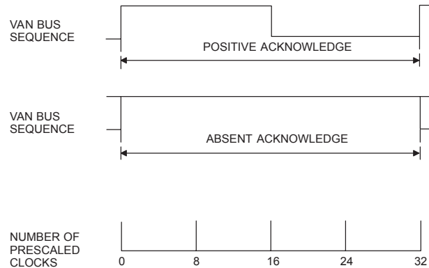
Figure 16. Acknowledge Sequences
