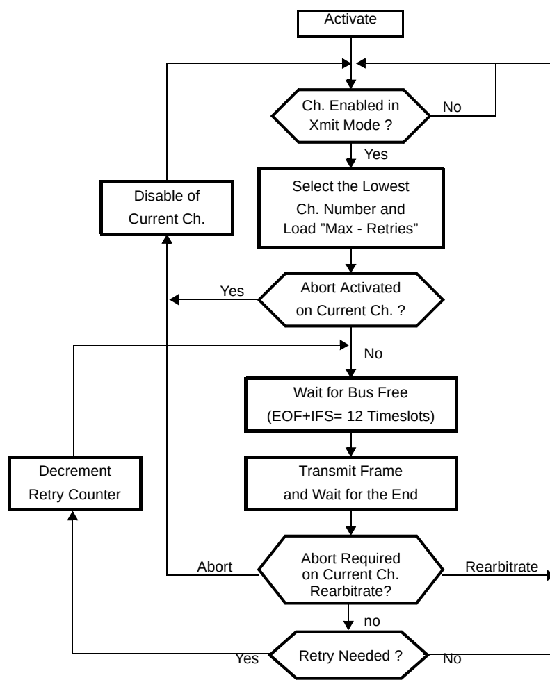
Figure 30. Transmit Function
