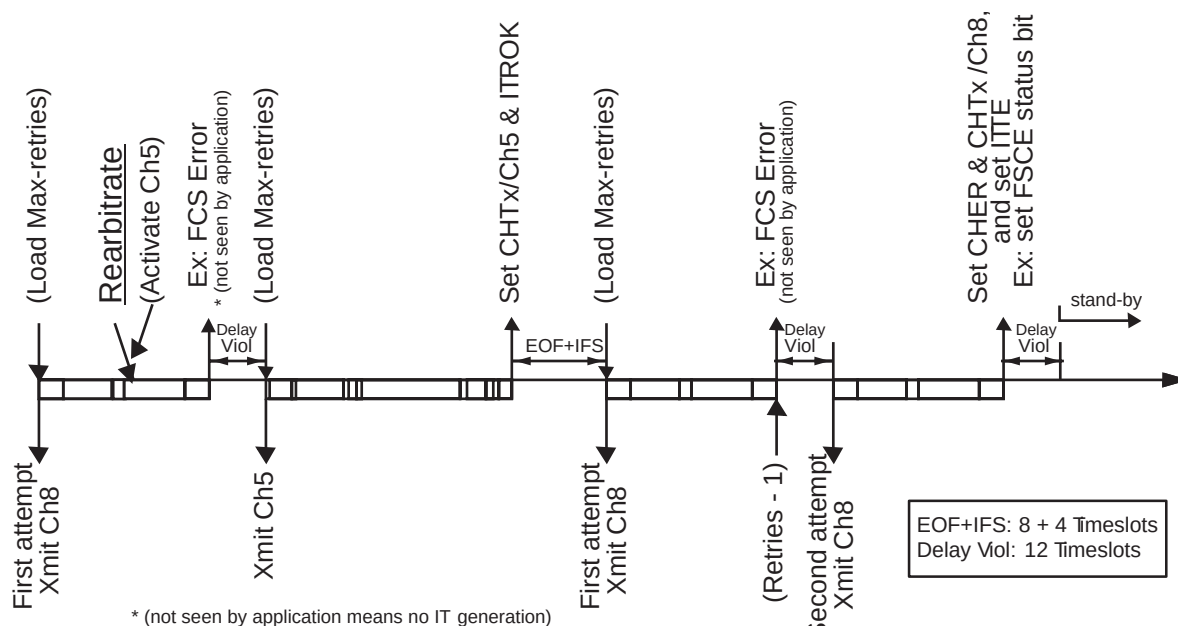
Figure 31. Rearbitrate Example
