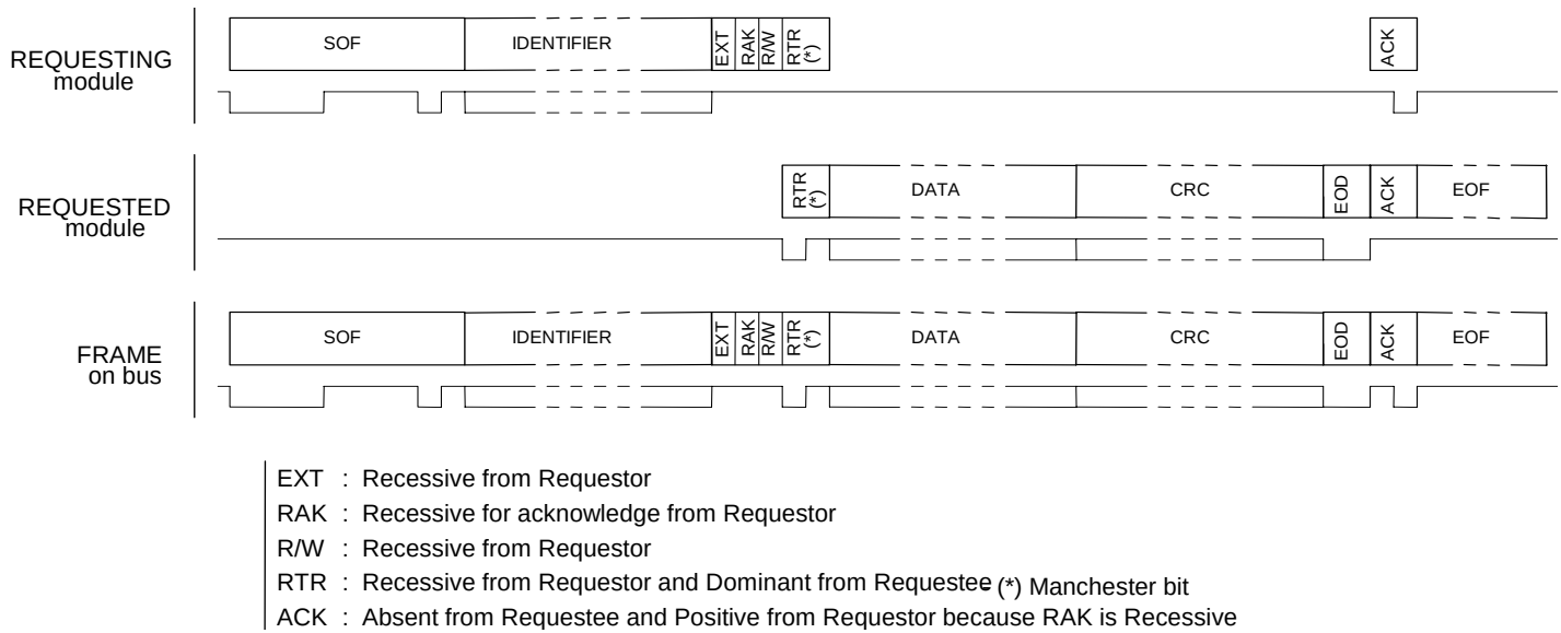
Figure 19. Reply Request Frame with Deferred Reply
