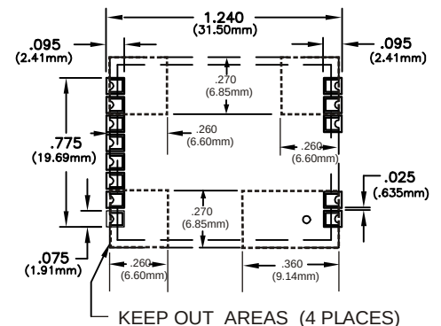
SUGGESTED PAD LAYOUT (TOP VIEW)
