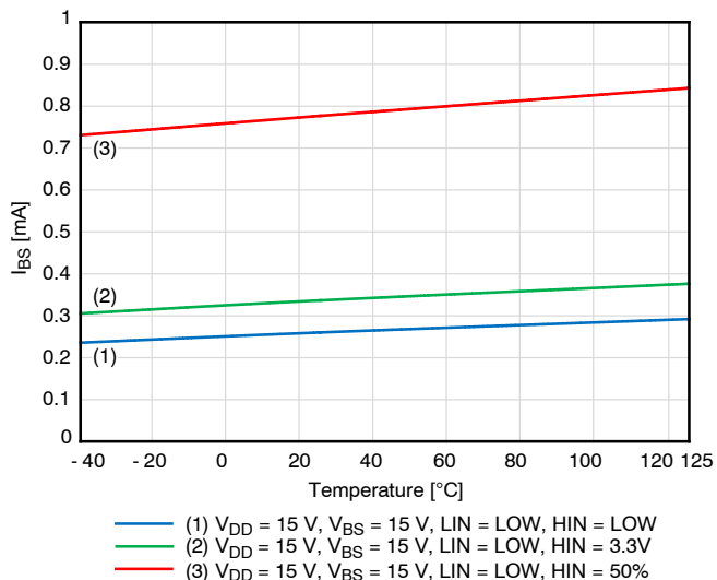
Figure 12. I_{BS} Supply Current V_{BS} = 15 V
