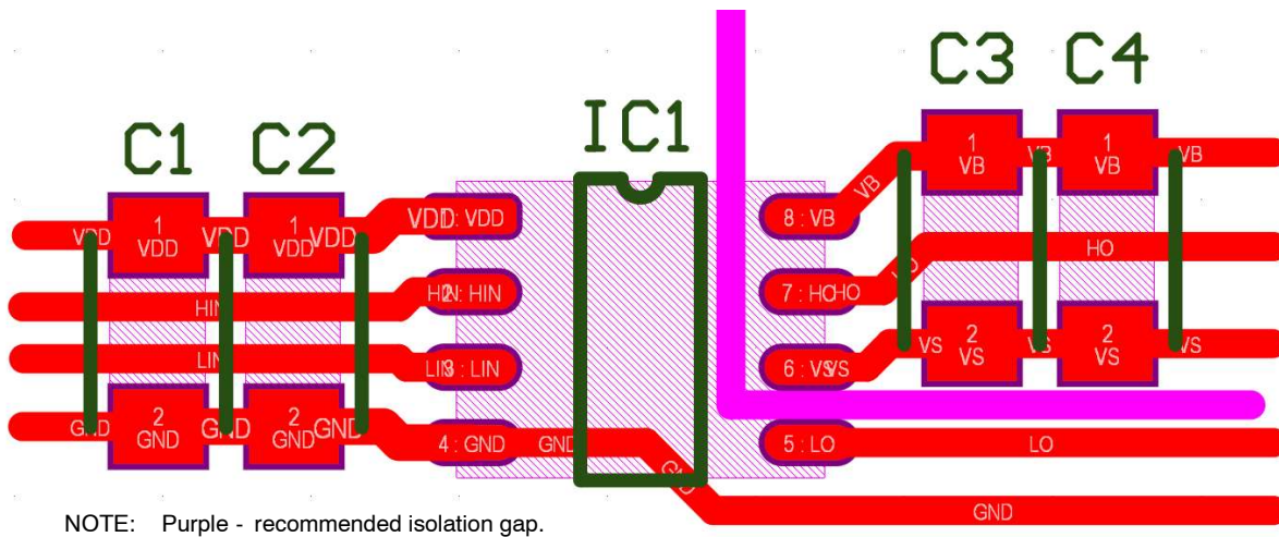
Figure 33. Recommended Layout
