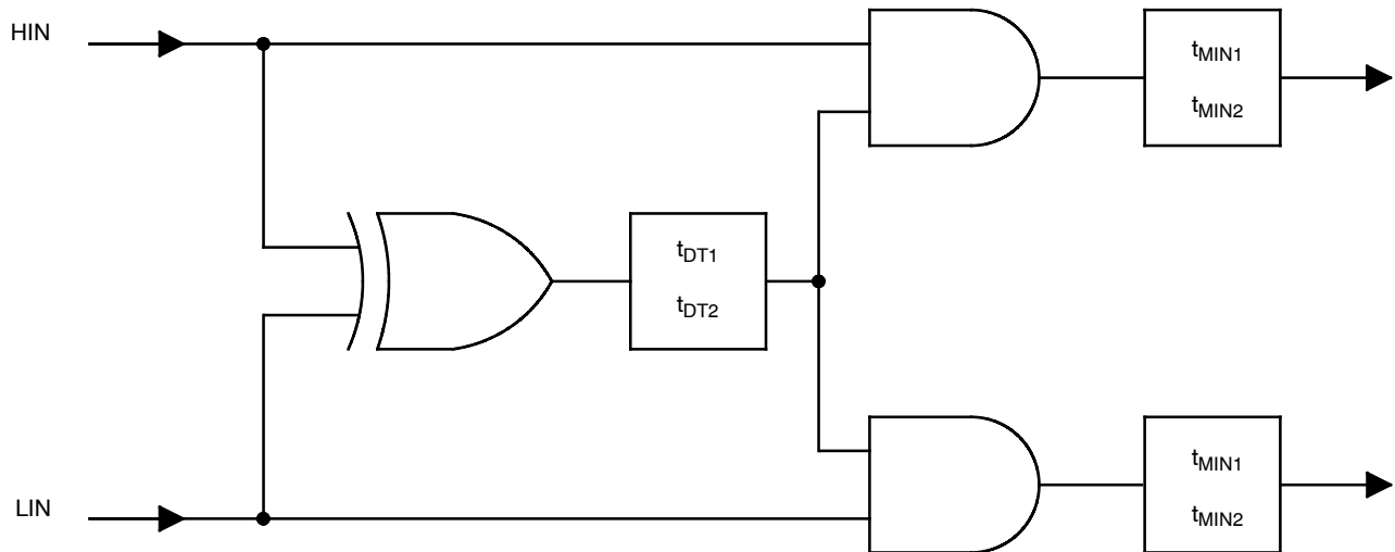
Figure 7. Input Circuit
