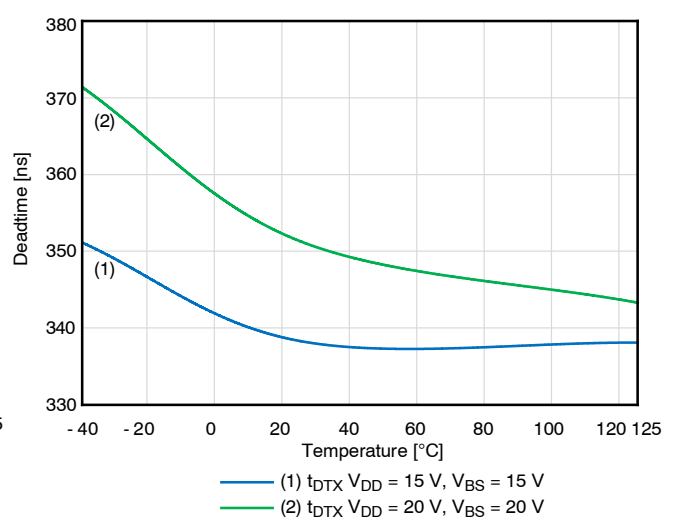
Figure 25. Deadtime
