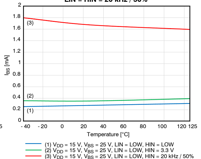
Figure 13. I_{BS} Supply Current V_{BS} = 25 V
