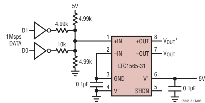
Simple Pulse Shaping Circuit for Single 5V Operation, 2Mbps (1Mps) 4 Level Data
