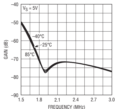
Stopband Gain vs Frequency Over Temperature
