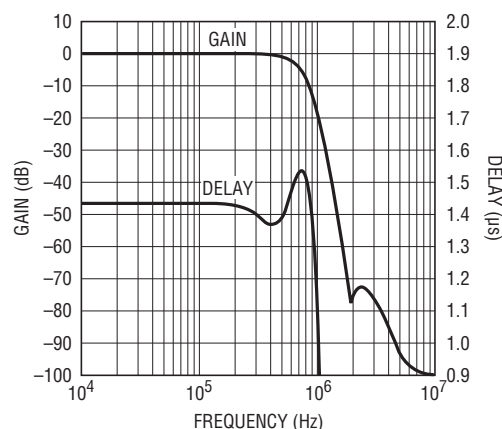
Frequency Response
