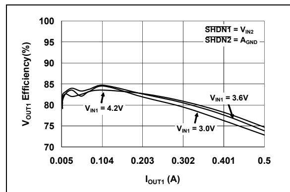
FIGURE 2-6: V_{OUT1} Output Efficiency vs. I_{OUT1} ( V_{OUT1} = 1.2V ).
