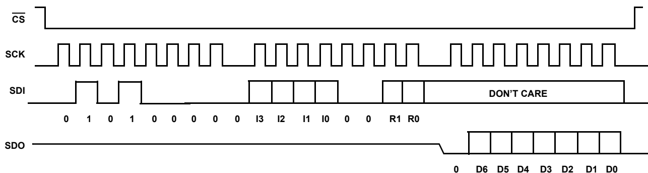
FIGURE 17. THREE BYTE READ SEQUENCE
