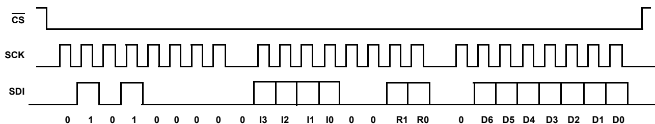
FIGURE 16. THREE BYTE WRITE SEQUENCE
