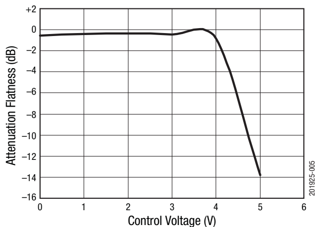
Figure 5. Attenuation Flatness vs Control Voltage ( f = 2.1\text{ to }3.1\text{ GHz} )
