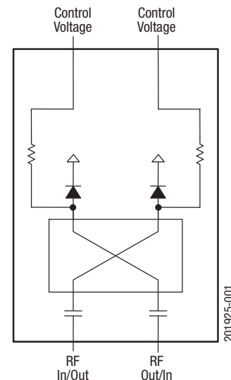
Figure 1. SKY12233-11 Block Diagram
