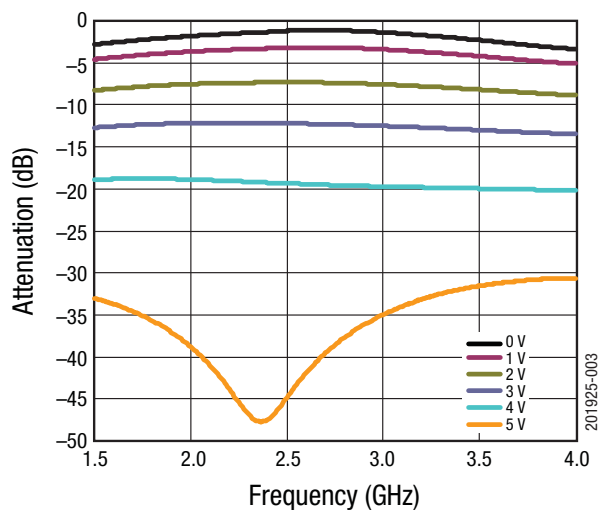
Figure 3. Attenuation vs Frequency Over Control Voltage
