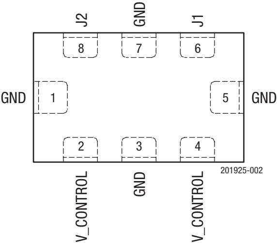
Figure 2. SKY12233-11 Pinout (Top View)
