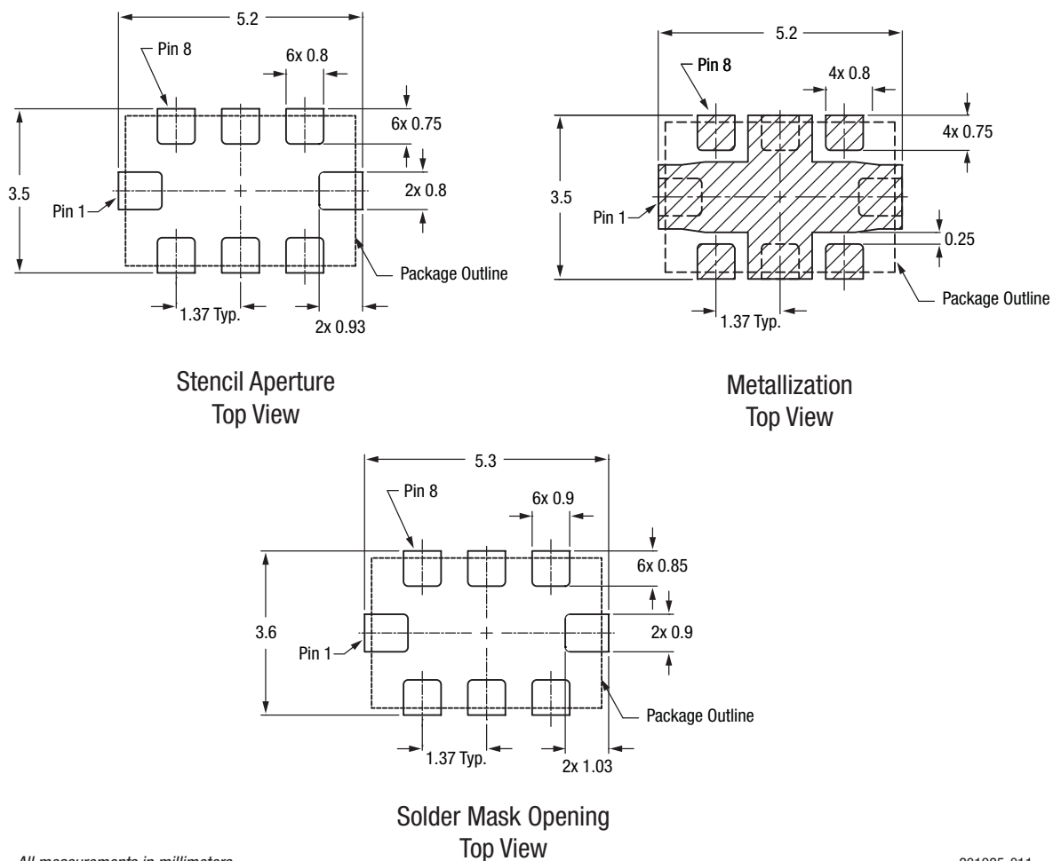
Figure 11. SKY12233-11 PCB Layout Footprint
