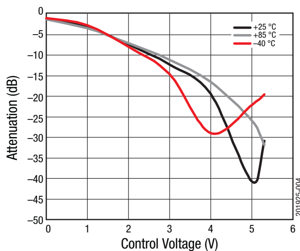
Figure 4. Attenuation vs Control Voltage Over Temperature ( f = 2.6\text{ GHz} )
