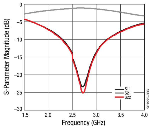
Figure 6. S-Parameter Magnitude vs Frequency
