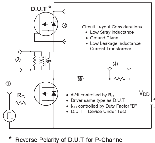
Fig 17. Diode Reverse Recovery Test Circuit for P-Channel HEXFET® Power MOSFETs
