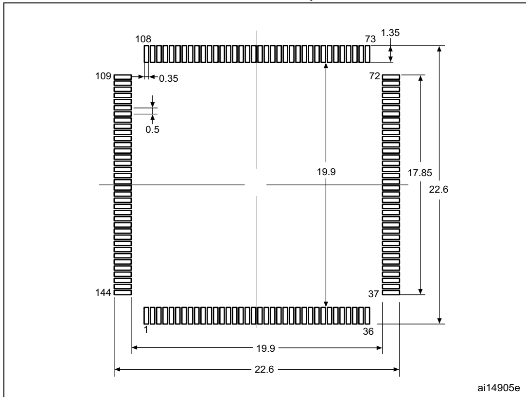
Figure 76. LQFP144, 20 x 20 mm, 144-pin low-profile quad flat package recommended footprint
