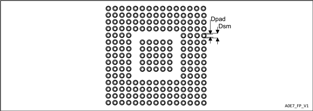
Figure 78. UFBGA176+25, 10 x 10 x 0.65 mm, ultra fine-pitch ball grid array package recommended footprint
