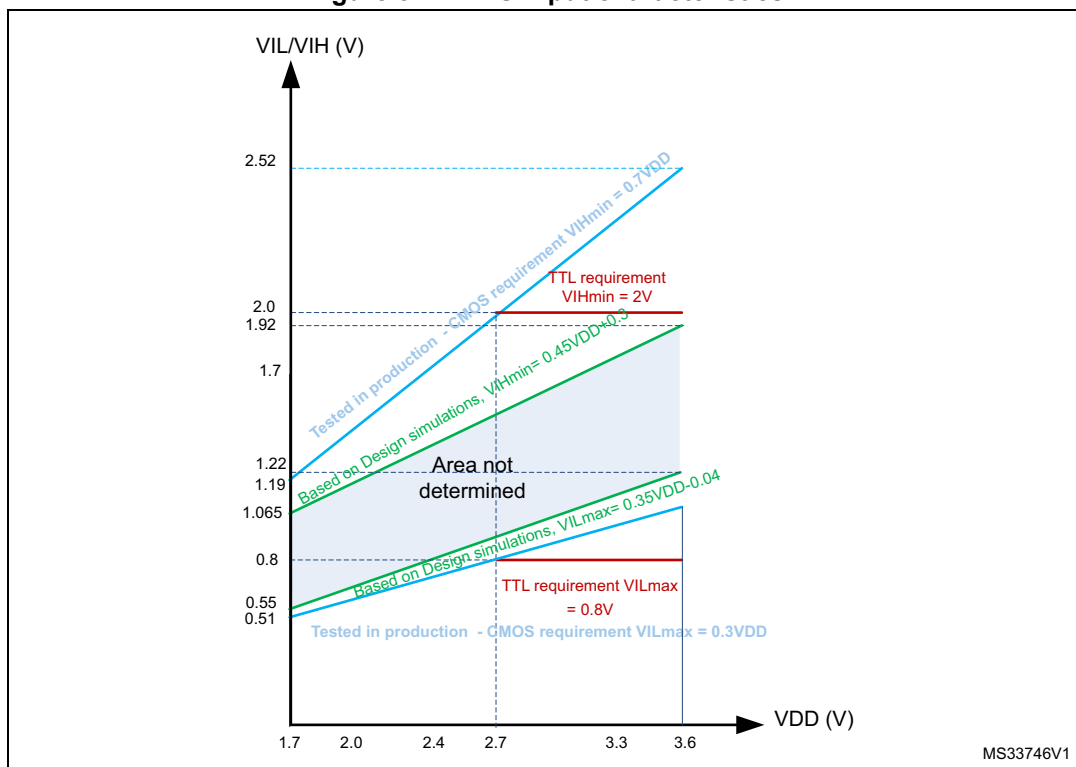
Figure 32. FT I/O input characteristics
