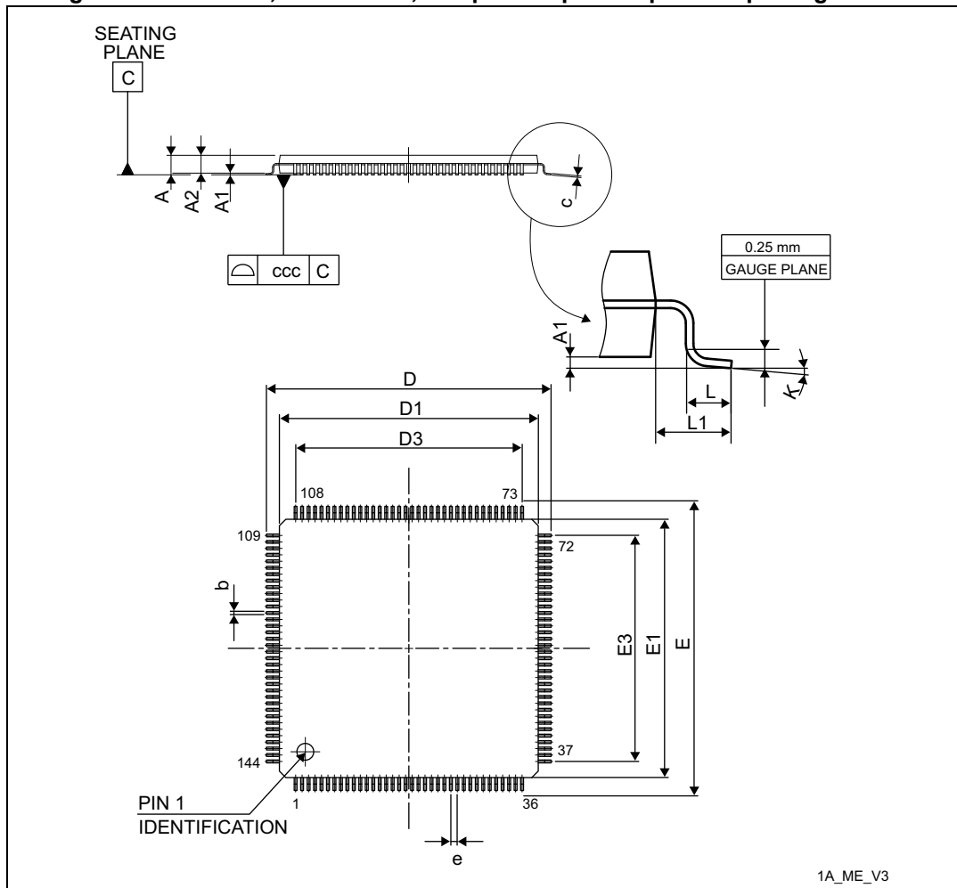
Figure 75. LQFP144, 20 x 20 mm, 144-pin low-profile quad flat package outline
