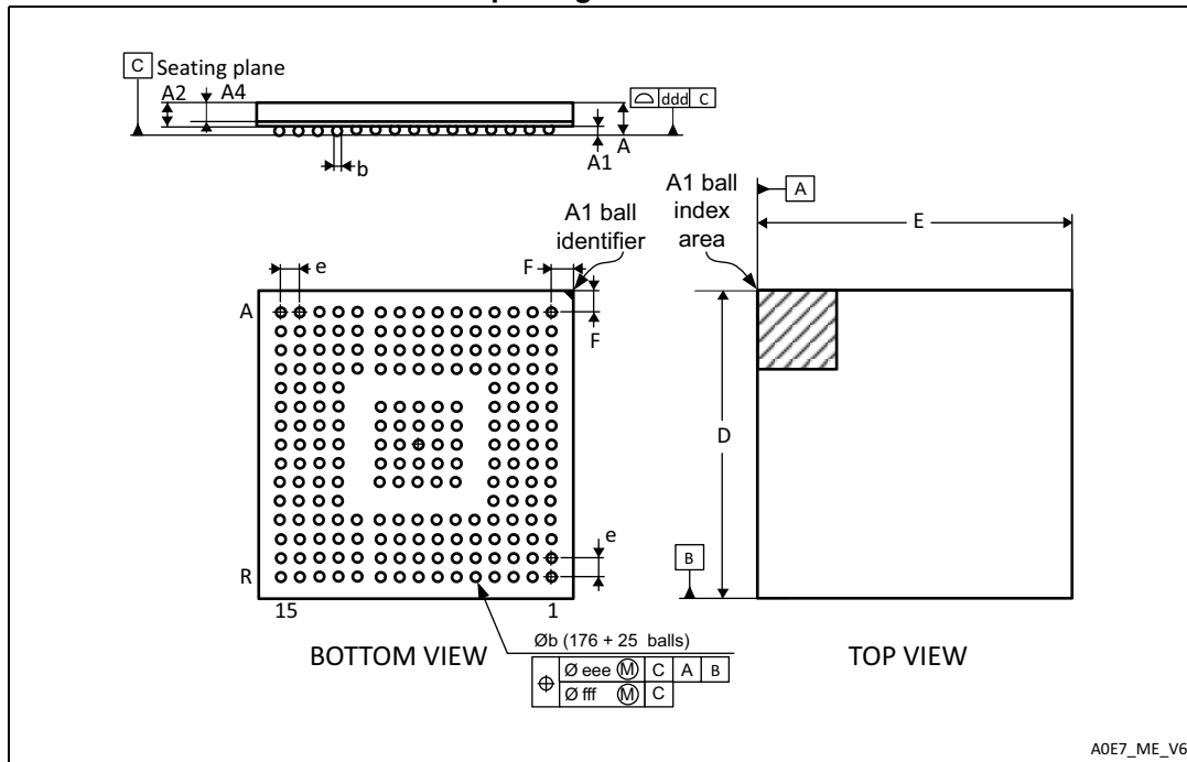
Figure 77. UFBGA 176+25, 10 × 10 × 0.65 mm ultra thin fine-pitch ball grid array package outline
