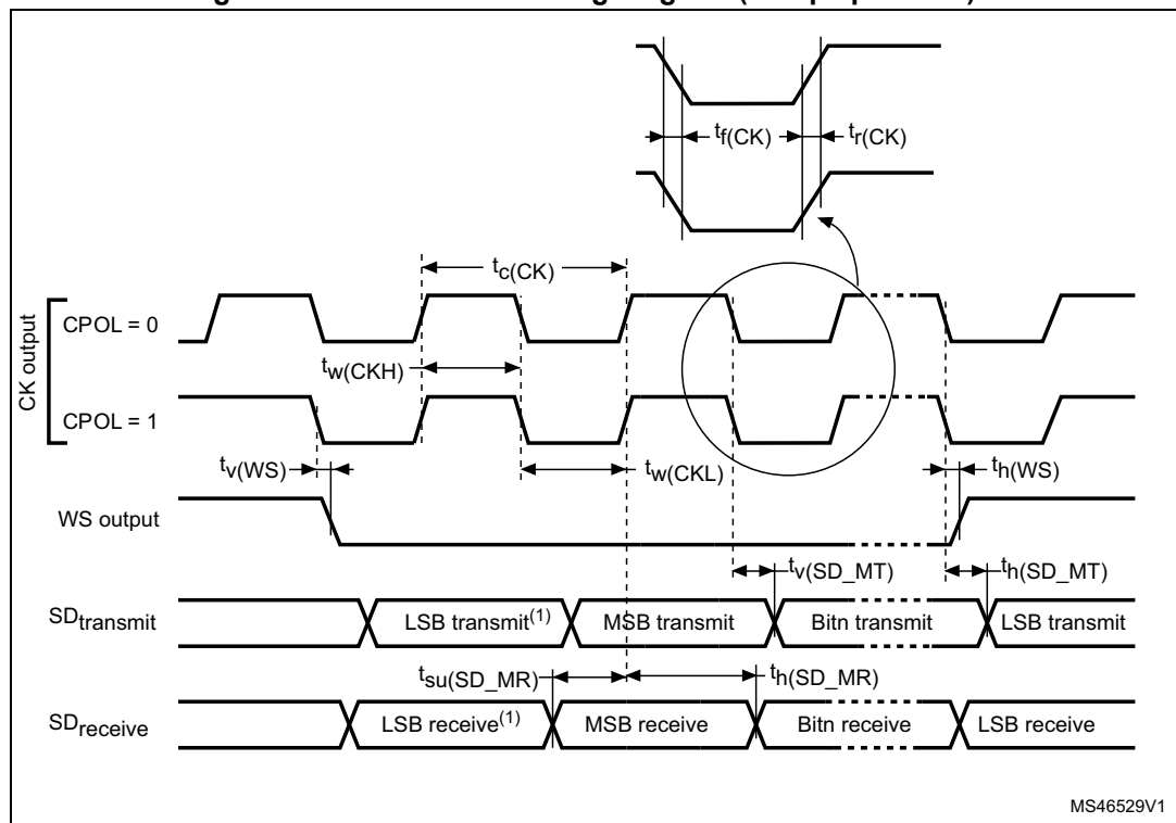
Figure 44. I 2 S controller timing diagram (Philips protocol) (1)
