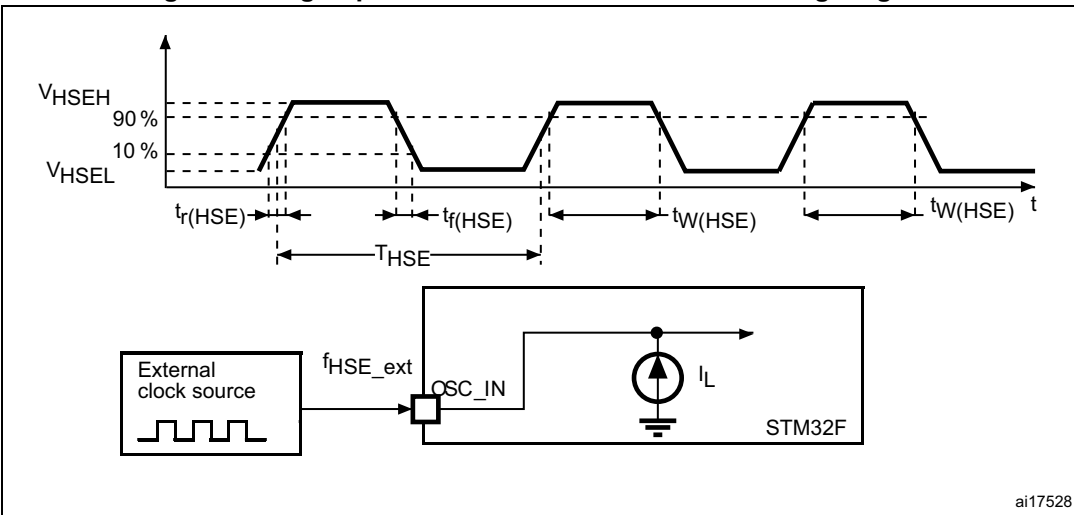
Figure 24. High-speed external clock source AC timing diagram
