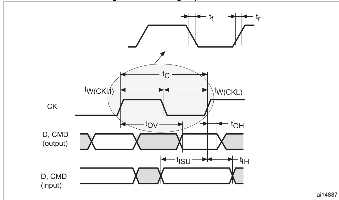
Figure 71. SDIO high-speed mode
