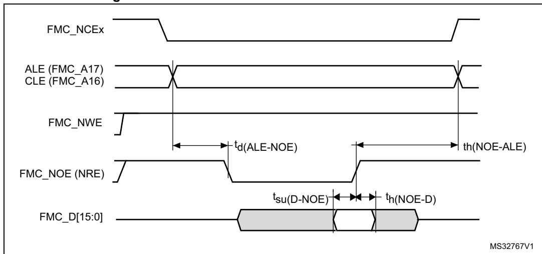
Figure 60. NAND controller waveforms for read access
