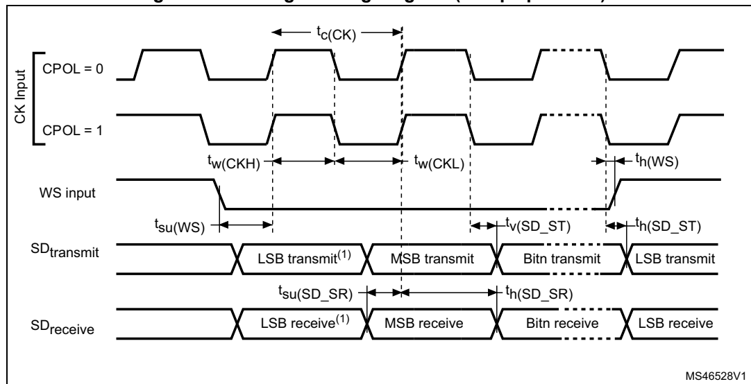
Figure 43. I 2 S target timing diagram (Philips protocol) (1)
