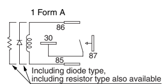
Schematic (Bottom view)
