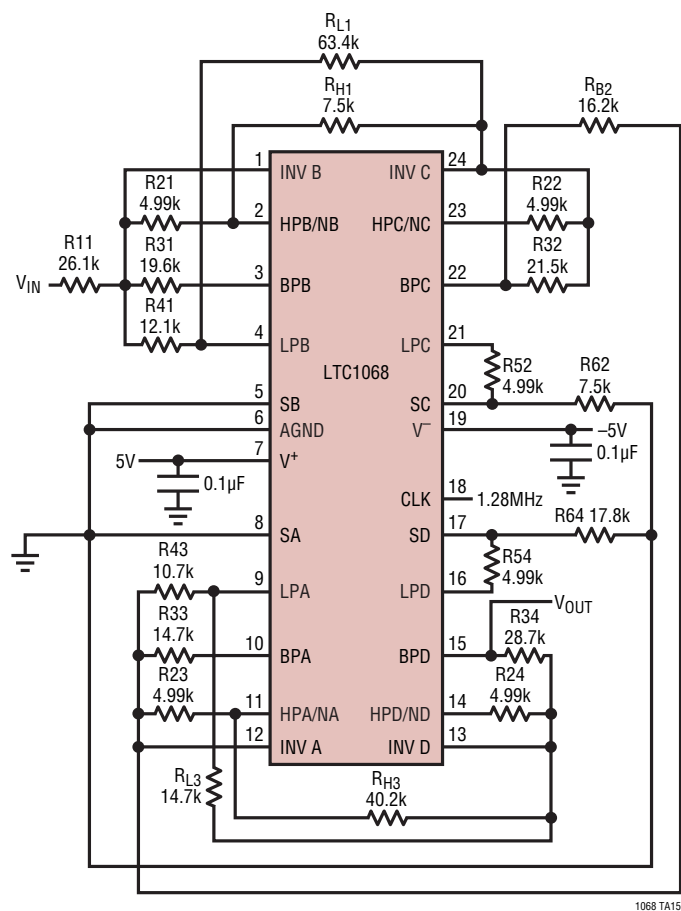
FilterCAD Custom Inputs for f_c = 10\text{kHz}
