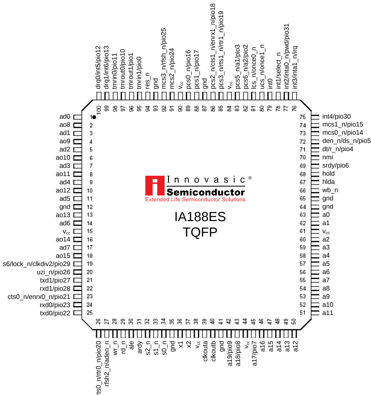
Figure 2. IA188ES TQFP Package Diagram
