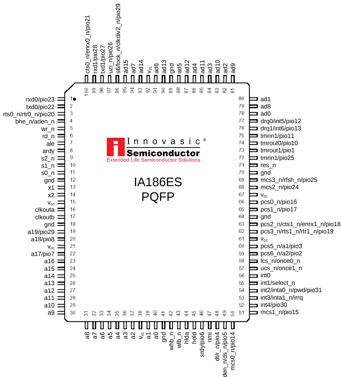
Figure 4. IA186ES PQFP Package Diagram
