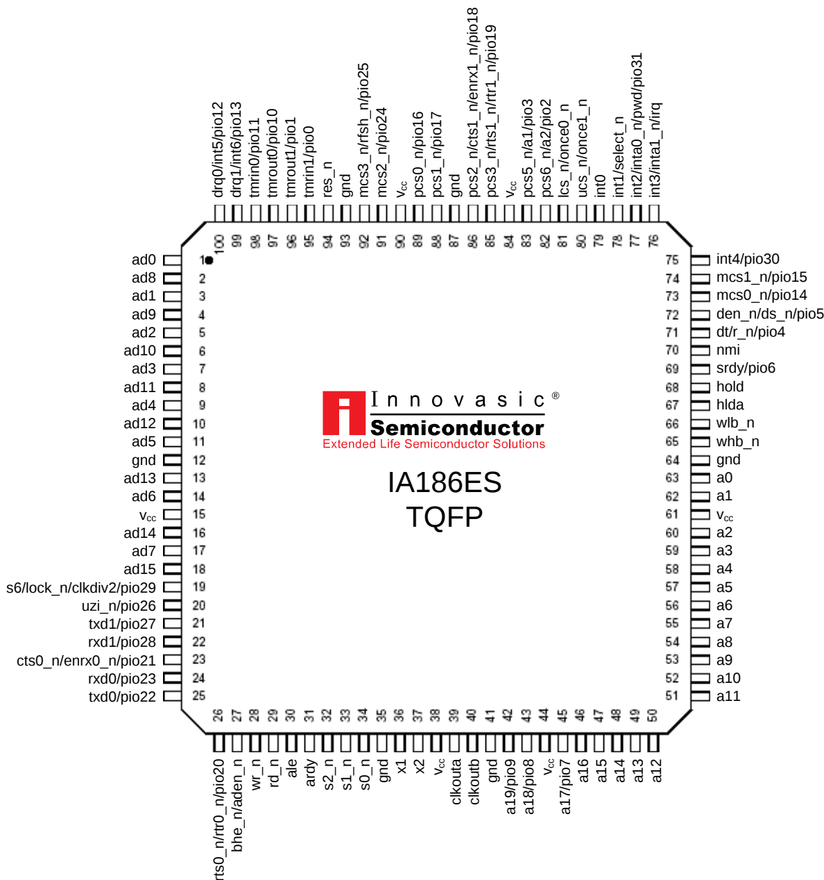
Figure 1. IA186ES TQFP Package Diagram
