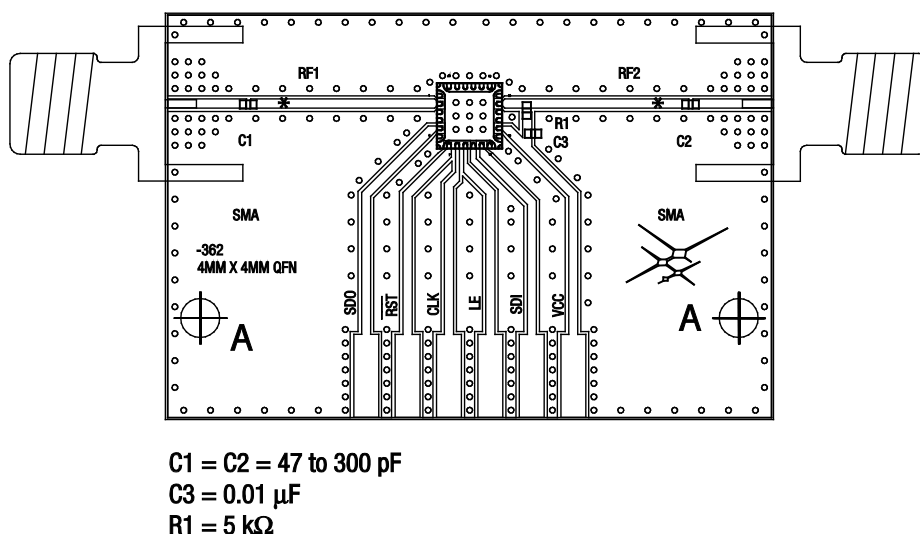
Figure 12. SKY12345-362LF Evaluation Board Assembly Diagram
