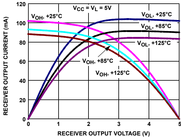
FIGURE 12. ISL3217XE RECEIVER OUTPUT CURRENT vs RECEIVER OUTPUT VOLTAGE
