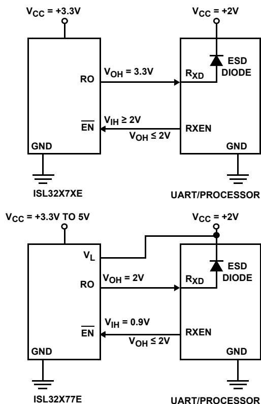
FIGURE 9. USING V L PIN TO ADJUST LOGIC LEVELS
