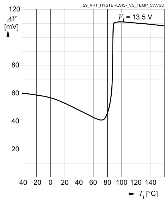
Reset Hysteresis versus Junction Temperature T_j (5V-Version)
