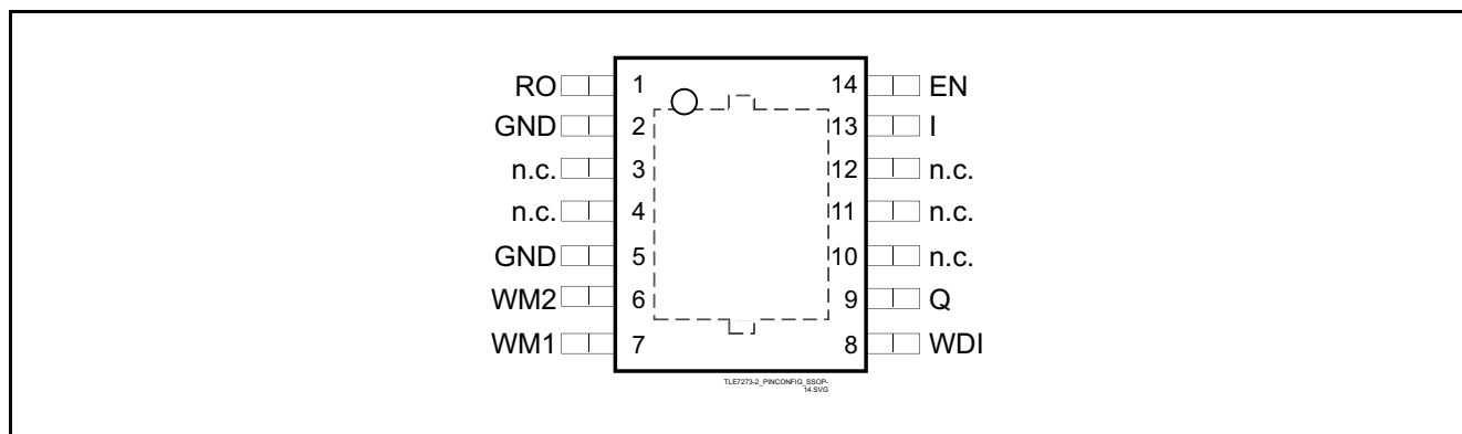
Figure 3 Pin Assignment PG-SSOP-14 Exposed Pad (top view)
