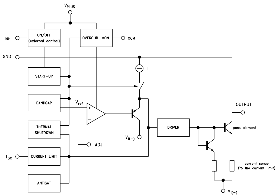
Figure 1. Block diagram
