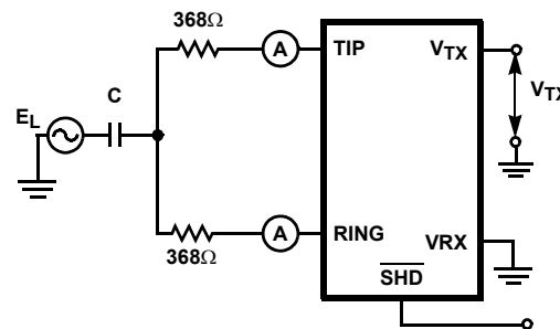
FIGURE 3B. LONGITUDINAL CURRENT LIMIT OFF-HOOK (ACTIVE)
