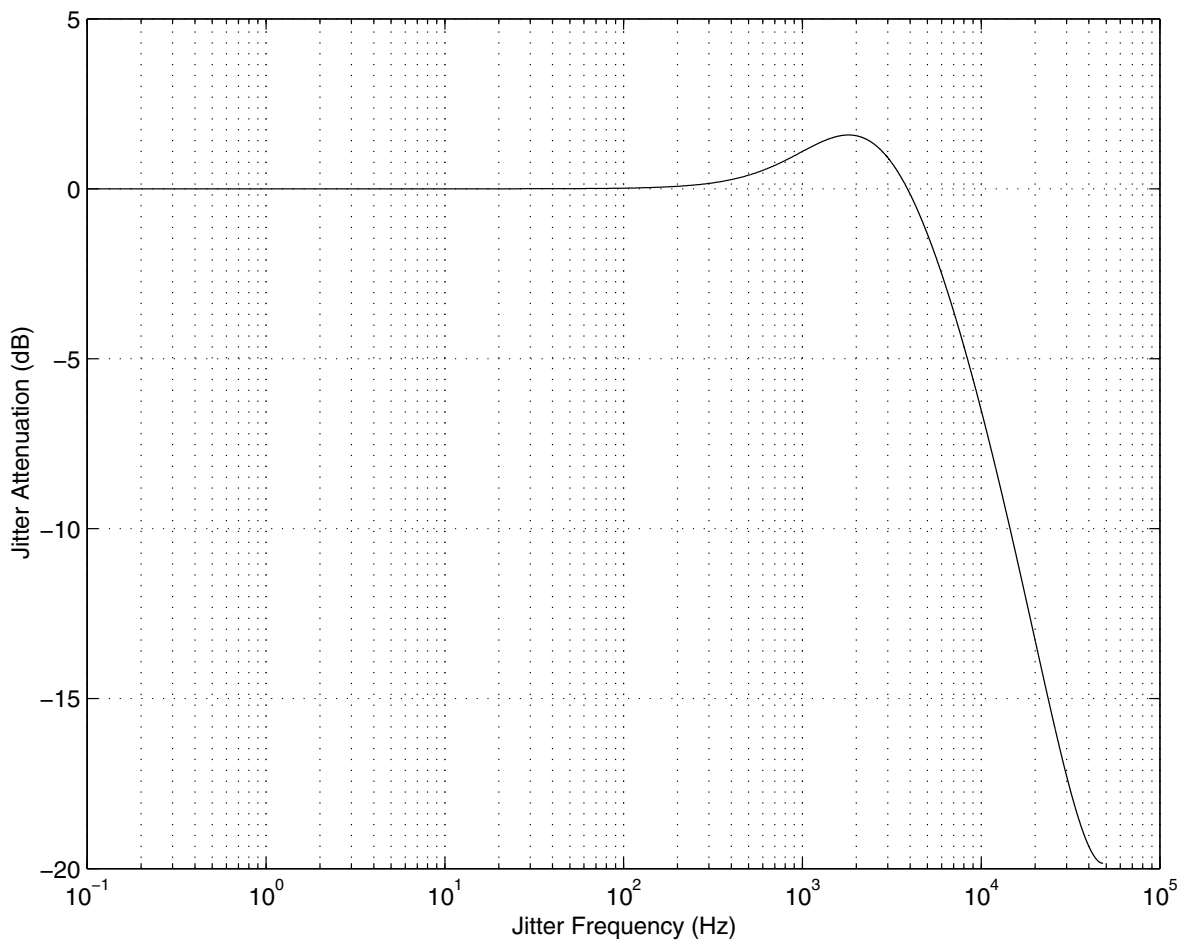
Figure 20. Jitter Attenuation Characteristics of PLL with Fs=32 to 96 kHz Filter Components
