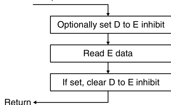
Figure 17. Flowchart for Reading the E Buffer
