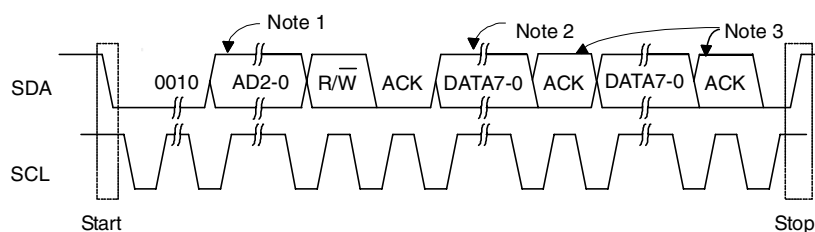
Figure 9. Control Port Timing in I 2 C Mode
