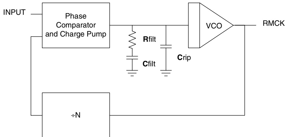
Figure 18. PLL Block Diagram
