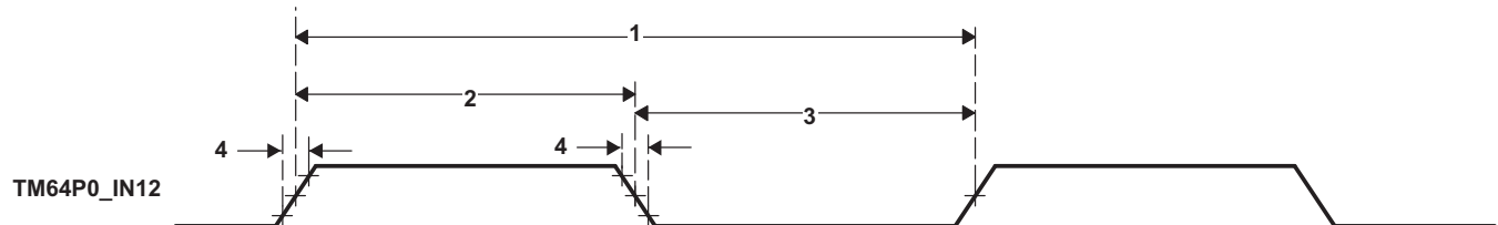
Figure 5-42. Timer Timing
