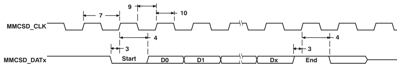
Figure 5-24. MMC/SD Host Read and Card CRC Status Timing
