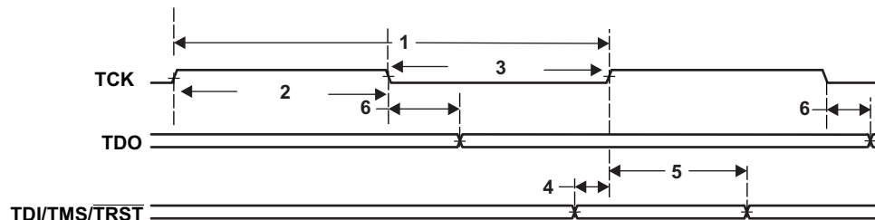
Figure 5-49. JTAG Test-Port Timing
