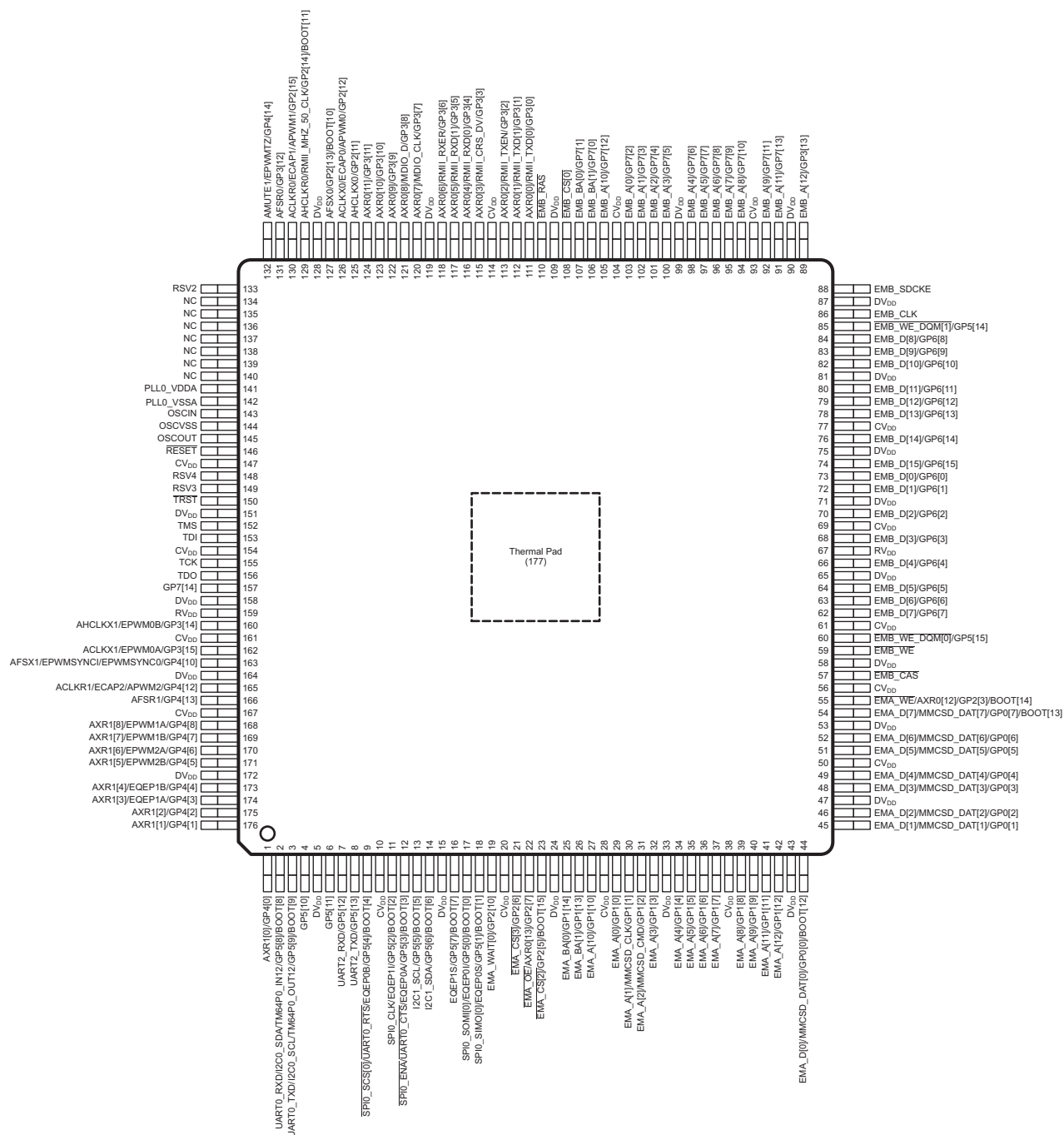
Figure 2-4. Pin Map (PTP)
