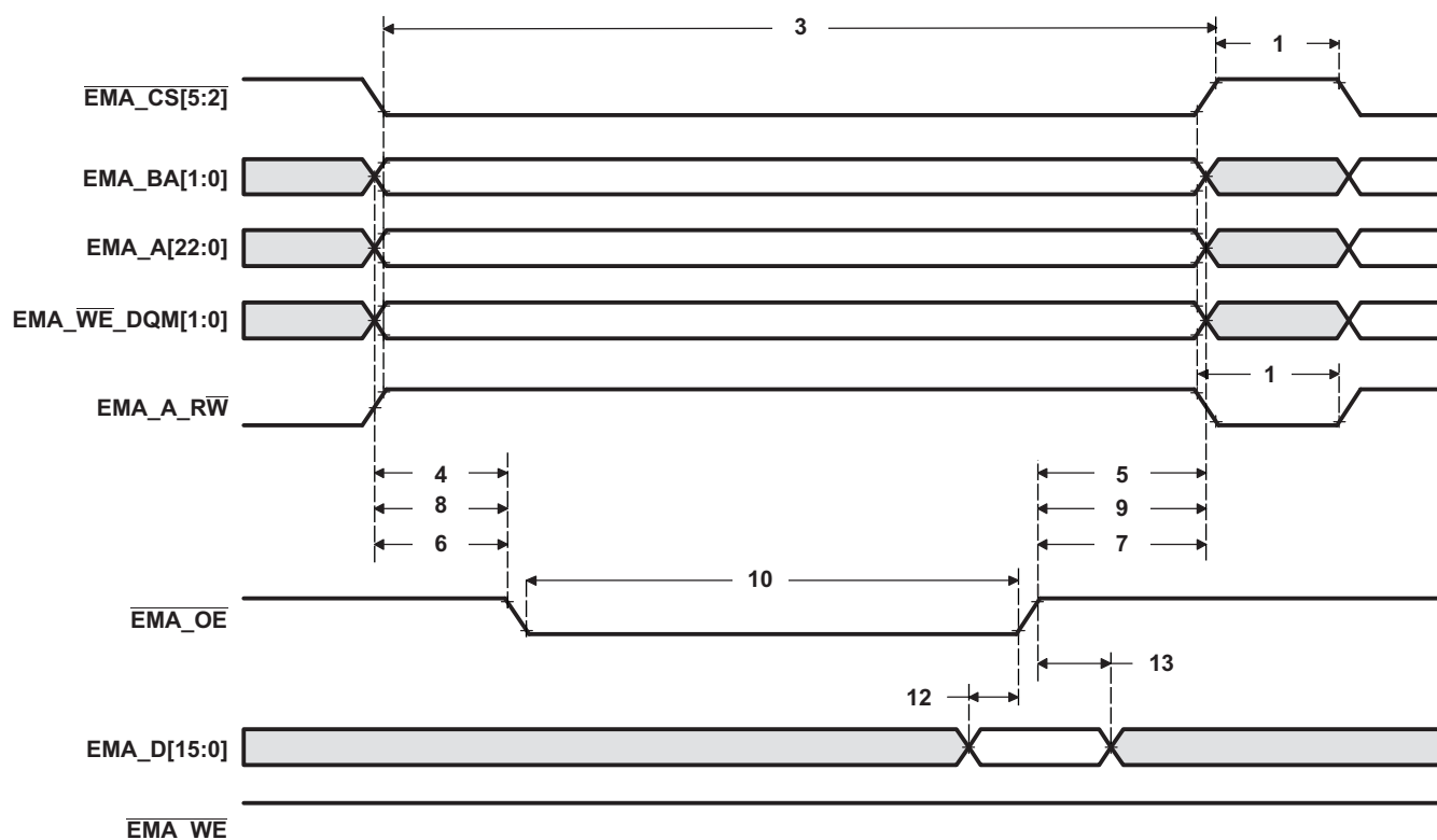
Figure 5-13. Asynchronous Memory Read Timing for EMIFA
