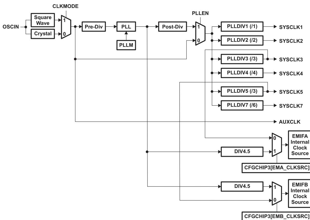
Figure 5-9. PLL Topology
