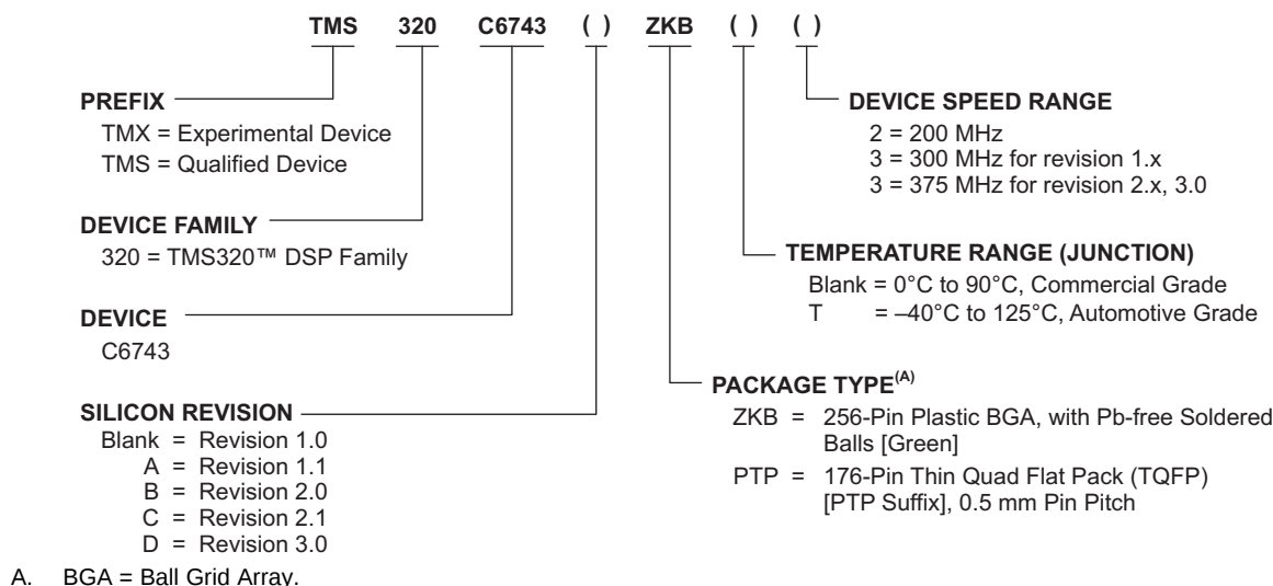
Figure 6-1. Device Nomenclature
