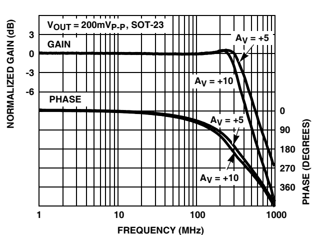
FIGURE 17. FREQUENCY RESPONSE
