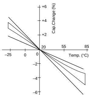
R200 (N750 \pm 300 ppm/ ^{\circ} C)
