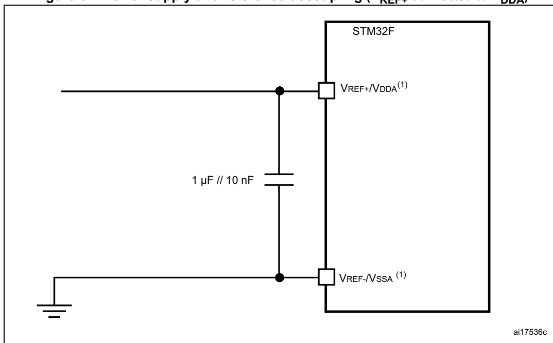
Figure 52. Power supply and reference decoupling ( V_{REF+} connected to V_{DDA} )
