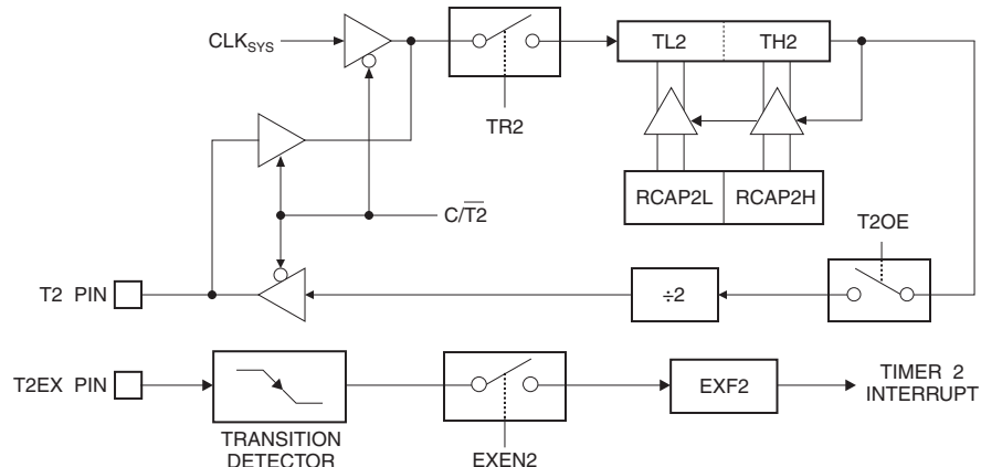
Figure 13-7. Timer 2 in Clock-out Mode
