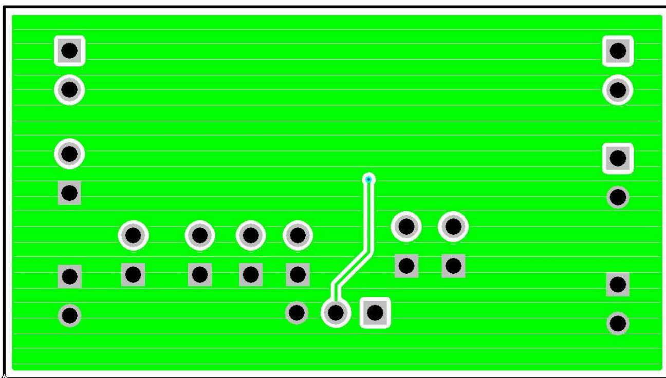
Figure 6. Bottom Side
