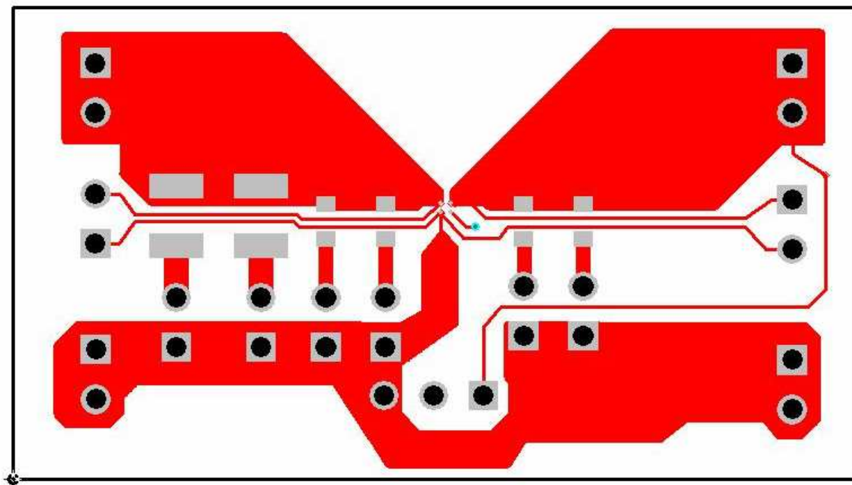
Figure 5. Top Side
