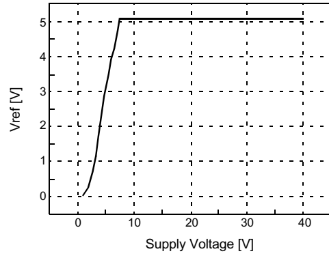
Reference Voltage
