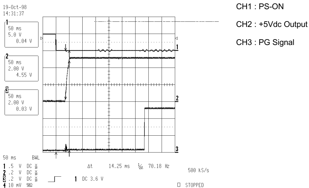
Figure 12. Rising Time of +5Vdc Output Voltage
