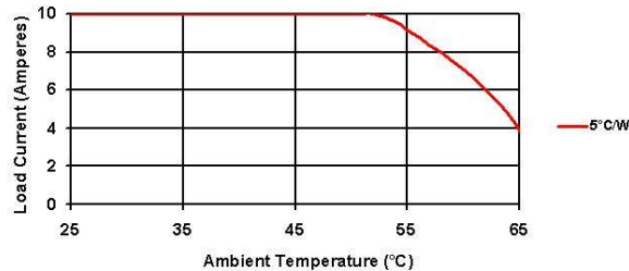
Derating Curve: DC60A10
