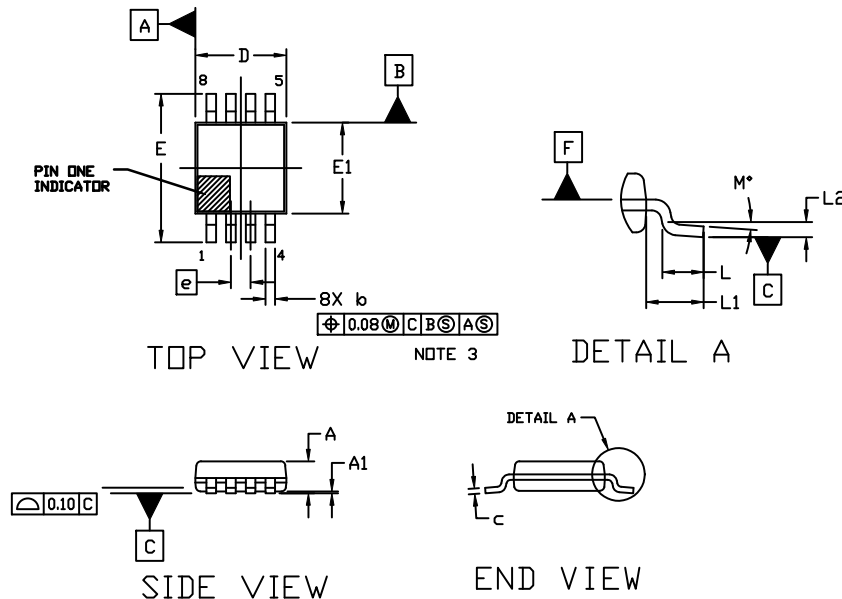
MSOP8 3.0x3.0 CASE 846AQ ISSUE O
