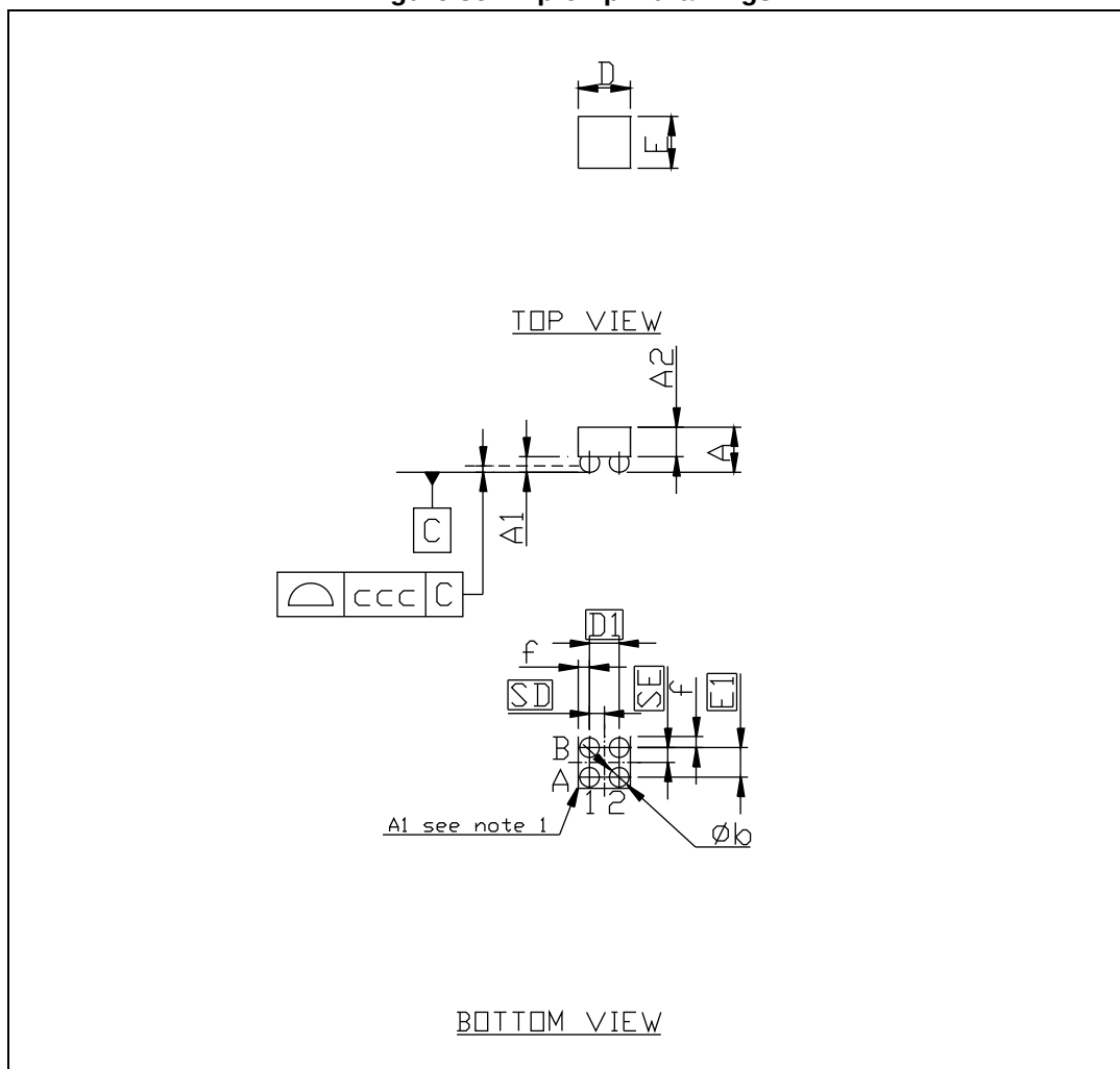
Figure 36. Flip-chip 4 drawings
