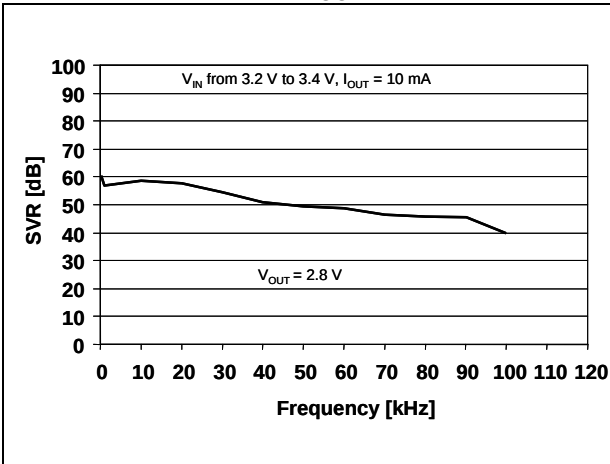
Figure 26. Supply voltage rejection vs. frequency ( V_{OUT} = 2.8 \text{ V} )
