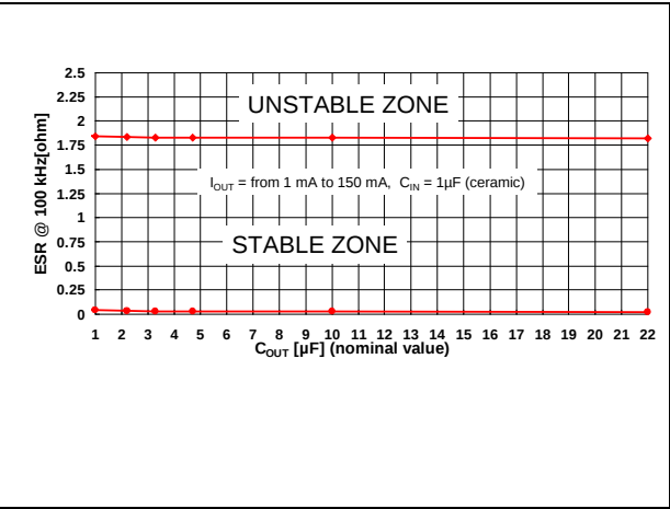
Figure 35. ESR required for stability with ceramics capacitors
