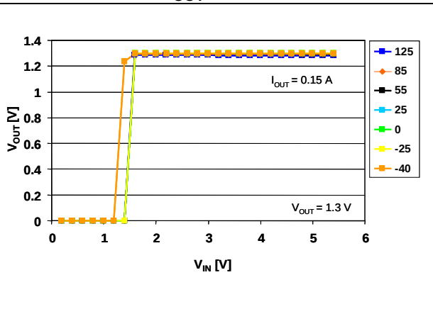
Figure 11. Output voltage vs. input voltage ( V_{OUT} = 1.3 V)
