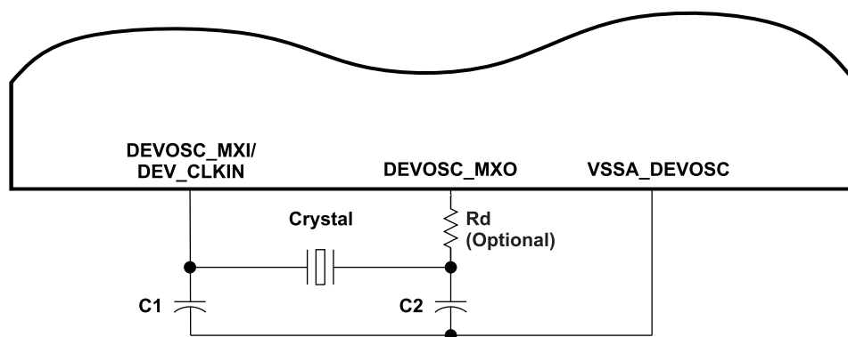
Figure 7-7. Device Oscillator
