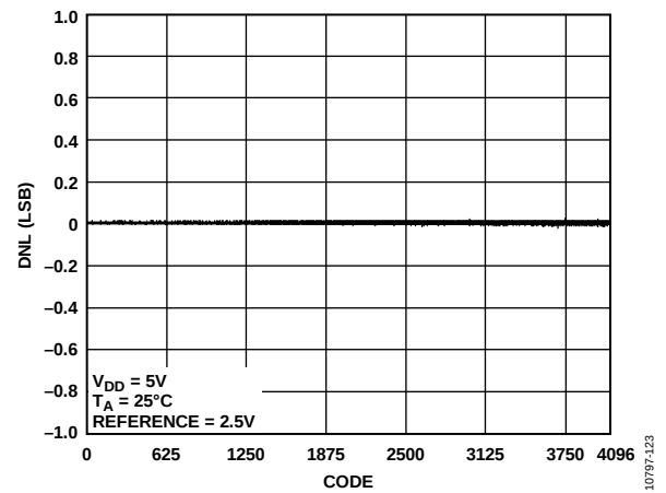
Figure 11. AD5684 DNL
