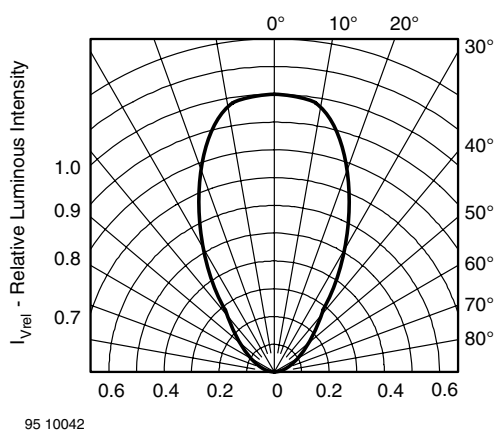
Figure 2. Rel. Luminous Intensity vs. Angular Displacement
