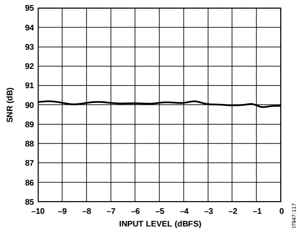
Figure 17. SNR vs. Input Level
