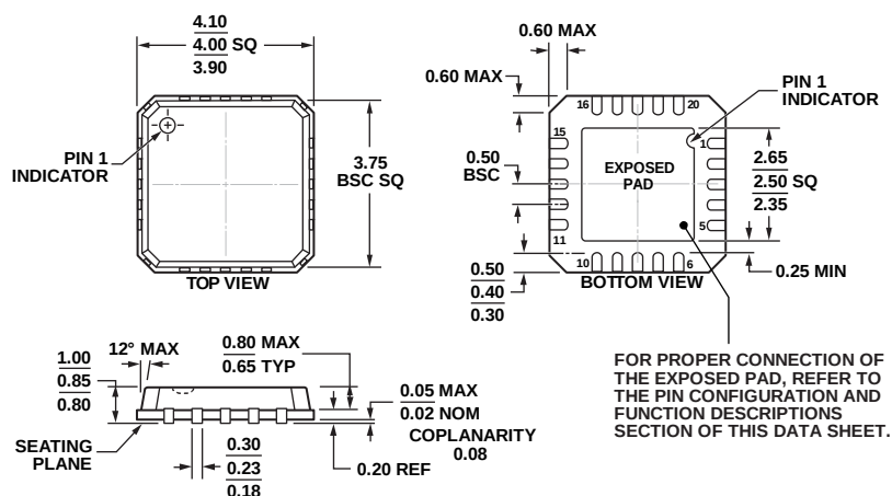
Figure 40. 20-Lead Lead Frame Chip Scale Package [LFCSP_VQ]
