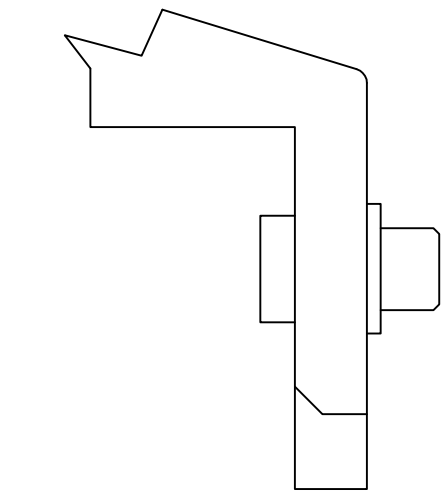
DETAIL T CLINCH NUT 8 PLC FOR -33,-34 AND -35 ONLY
