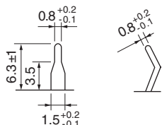
(Terminal dimensions)
