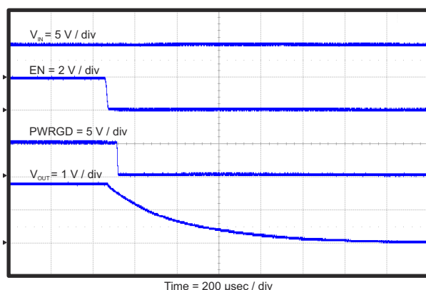
Figure 8-8. Power Down Relative To EN
