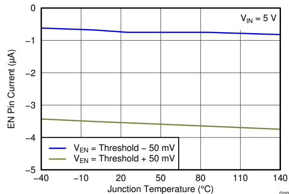
Figure 6-8. EN Pin Current vs Temperature
