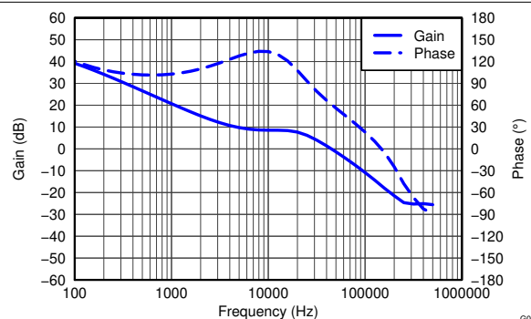
Figure 8-11. Closed Loop Response, V_{IN} = 5\text{ V} , I_{OUT} = 3.5\text{ A}
