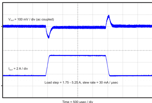
Figure 8-4. Transient Response, 3.5 A Step
