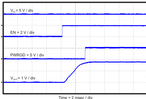
Figure 8-7. Power Up Relative To EN
