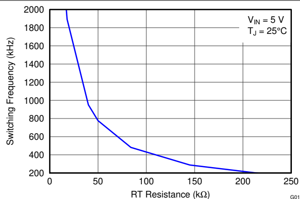
Figure 6-12. Switching Frequency vs R_T Resistance
