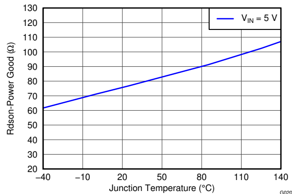
Figure 6-19. PWRGD Rdson vs Temperature
