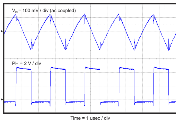
Figure 8-10. Input Ripple, I_{OUT} = 7\text{ A}
