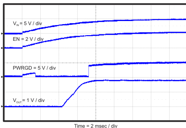
Figure 8-5. Power Up Relative To VIN
