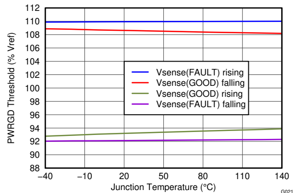
Figure 6-20. PWRGD Threshold vs Temperature
