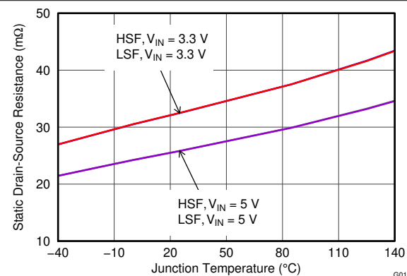
Figure 6-10. Rdson vs Temperature
