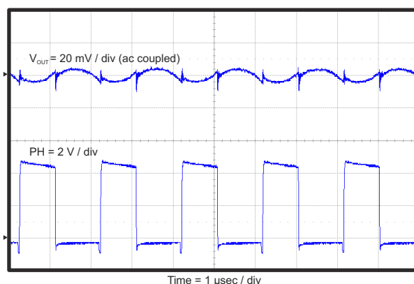
Figure 8-9. Output Ripple, I_{OUT} = 7\text{ A}
