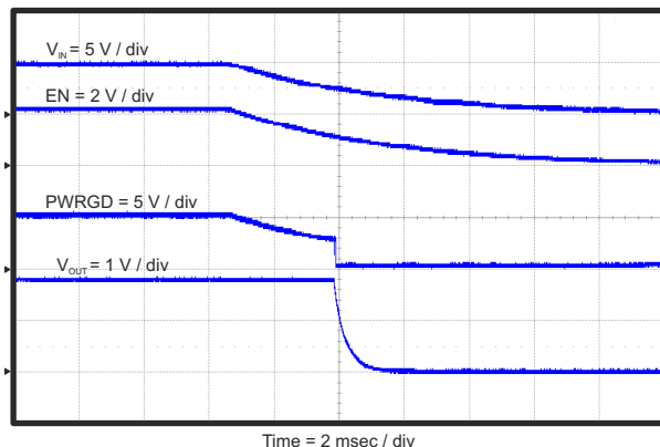
Figure 8-6. Power Down Relative To VIN
